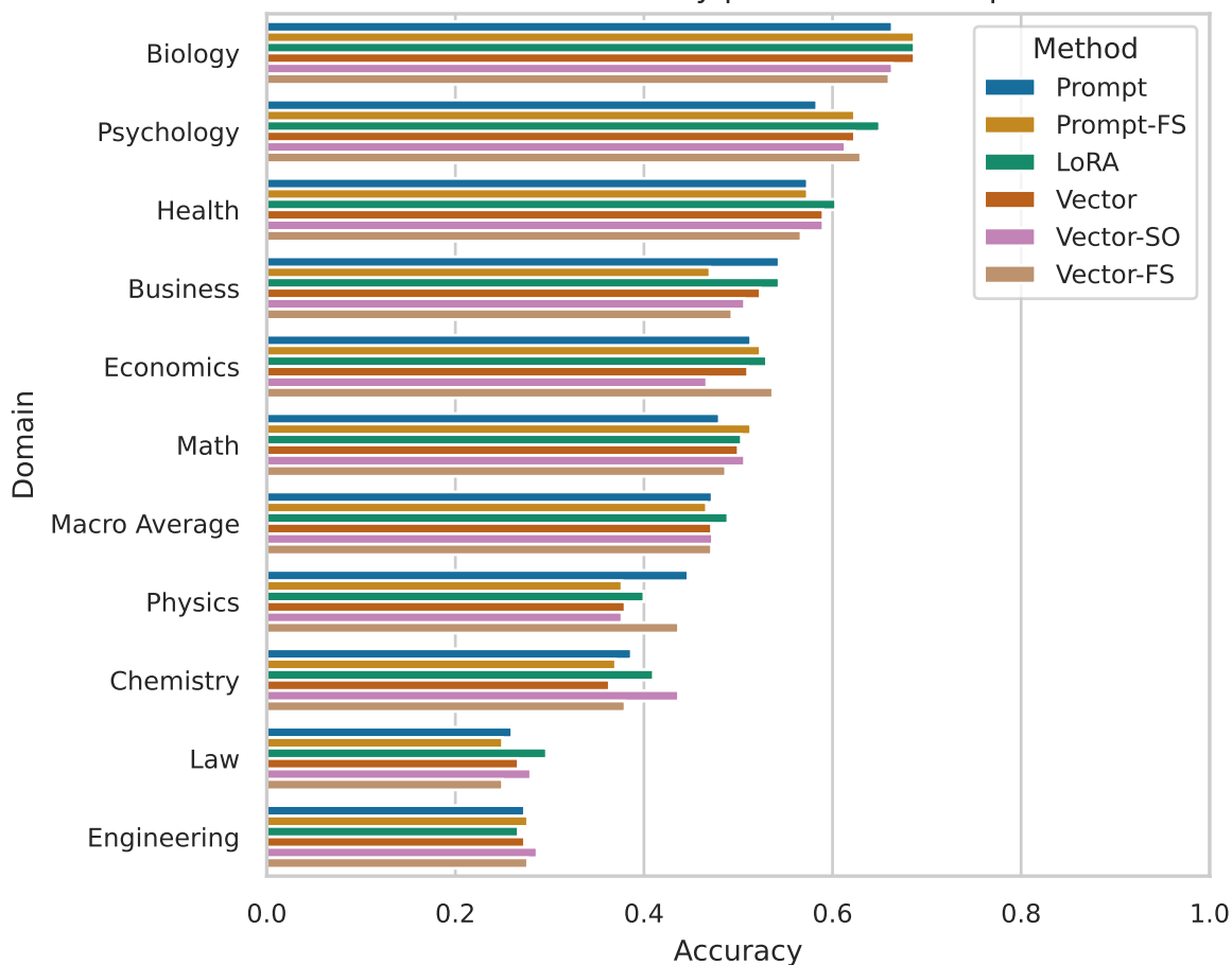
Model Accuracy per Dataset/Setup
