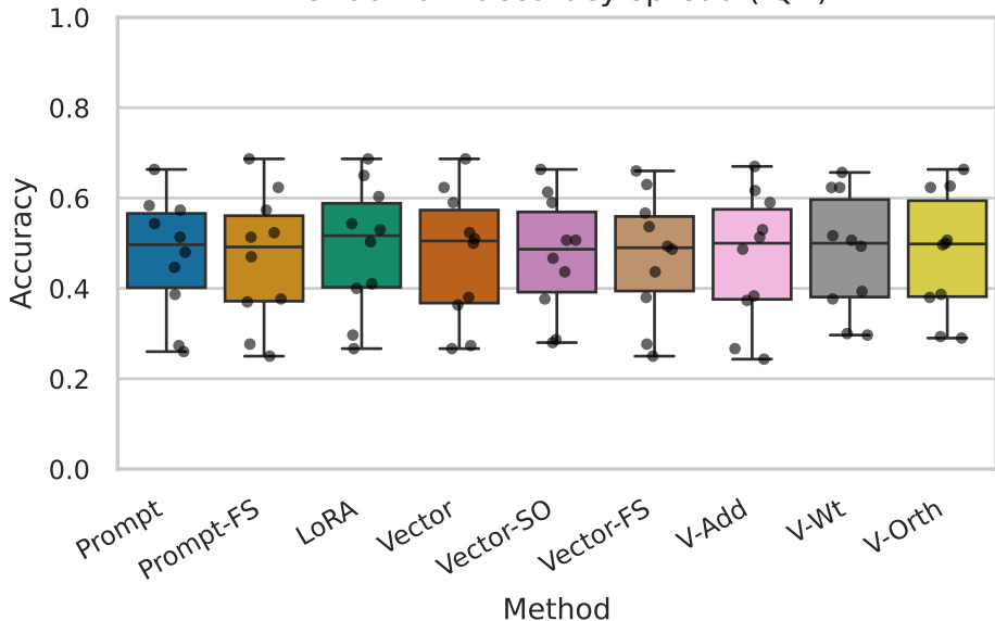
Per-domain accuracy spread (IQR)
