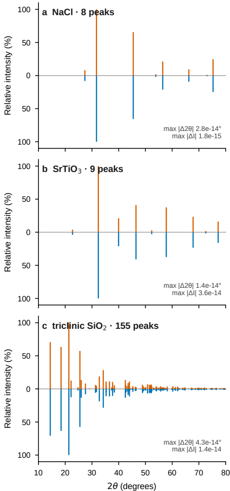
Powder lines: no broadening
