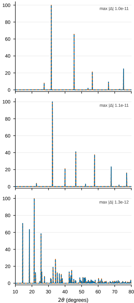
Both profiles: FWHM 0.1°
