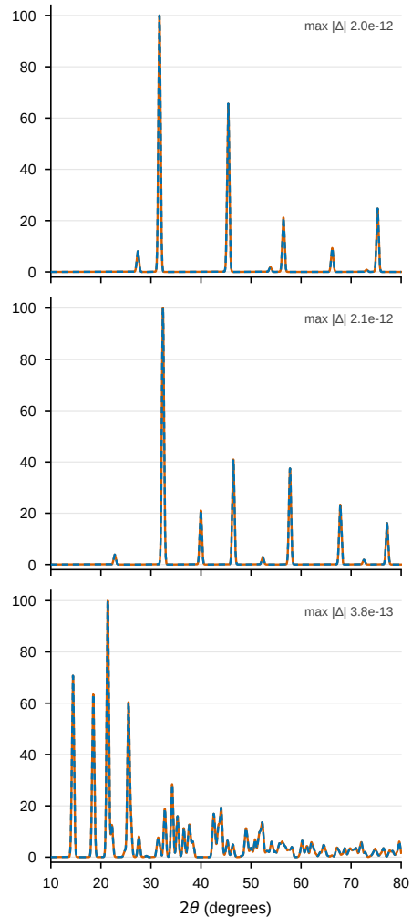
Both profiles: FWHM 0.5°
