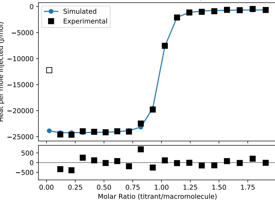
ITC Isotherm: simulation vs experiment
