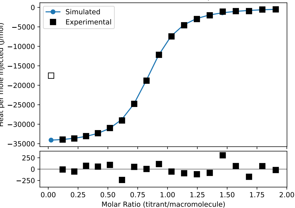
ITC Isotherm: simulation vs experiment
