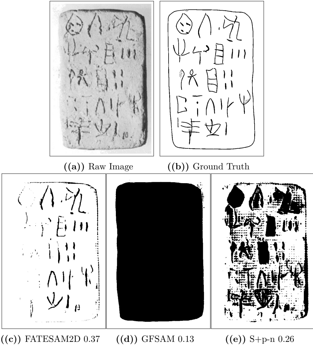
Figure 4.3: Visual comparison of output masks per ICL model and best SAM variant from Section 4.1.1 based on the segmentation of HT7a (easy), shown with Dice scores next to the raw image and ground truth. This is one of the instances where FATESAM2D performed better than the best zero-shot SAM implementation, but due to its tendency of undersegmentation, this was generally not the case.
