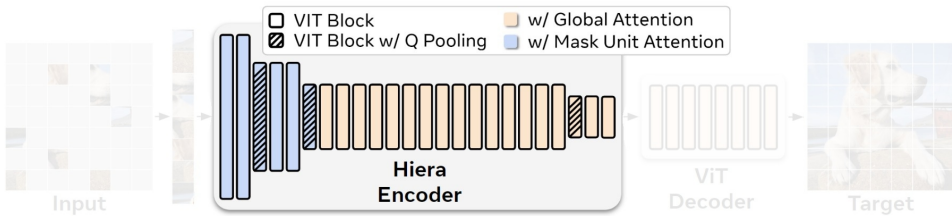
Figure 3.4: Architecture of Hiera, adapted from Ryali et al. (2023).
