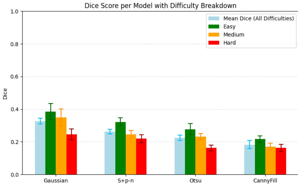
Figure 4.4: Dice score comparison of all models on the evaluation dataset.
