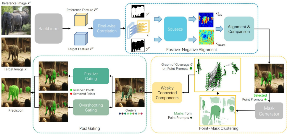
Figure 3.6: Architecture of GFSAM, from A. Zhang et al. (2024).
