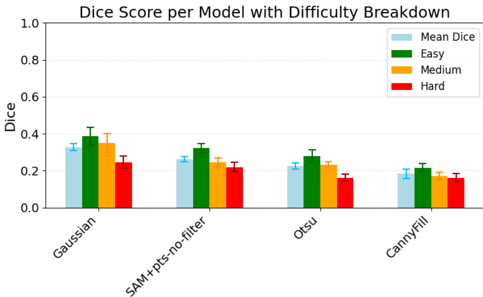
Figure 4.4: Mean Dice scores of the classical baselines; CannyFill (0.183), Otsu (0.224), and Gaussian (0.327), compared to the best SAM variant found in Section 4.1.2 and Section 4.1.1, SAM+pts-no-filter (0.263). Split by difficulty. With error bars representing the standard error of the mean. Ordered descendingly from the left by mean performance.
