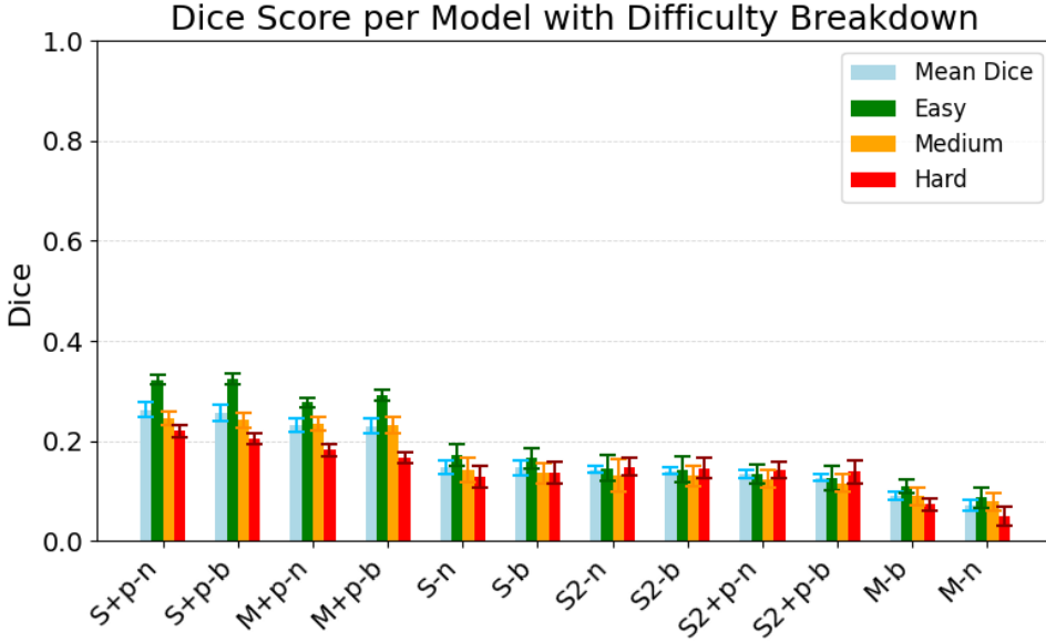
Figure 4.1: Mean Dice scores per SAM variant. Split by difficulty. With error bars representing the standard error of the mean. Ordered descendingly from the left by mean performance. The ablations evaluated were MobileSAM (M), SAM (S), and SAM2 (S2), with (+p) or without automatic point prompts, and with (b) or without (n) a bilateral pre-filter.
