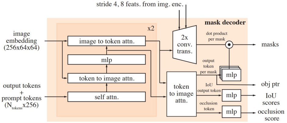
Figure 3.8: Architecture of SAM2's mask decoder, from Ravi et al. (2024).
