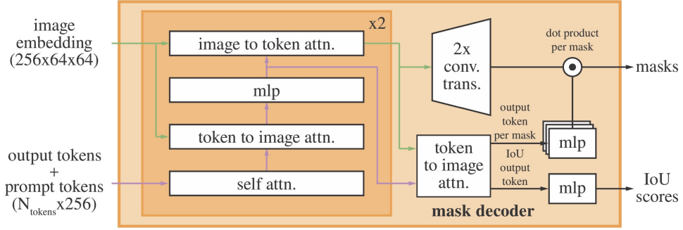
Figure 3.5: Architecture of SAM’s mask decoder, from Kirillov et al. (2023).
