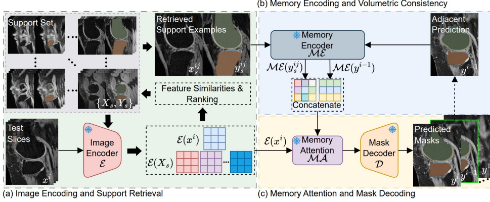
Figure 3.9: Architecture of FATESAM, from He et al. (2025b).
