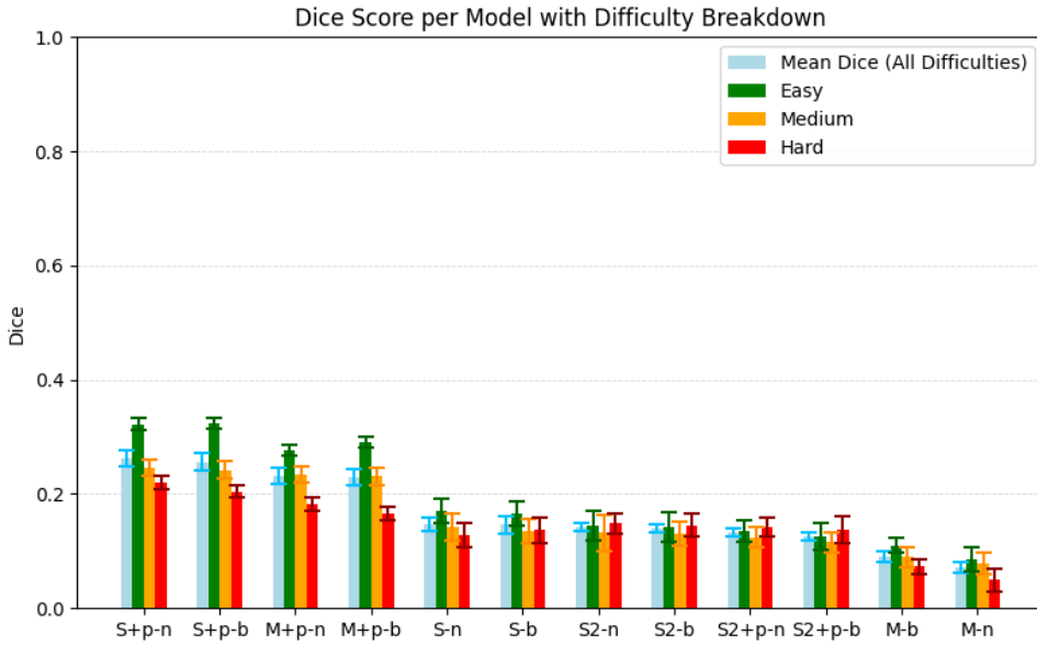
Figure 4.1: Dice Score performance per SAM variant. Split by difficulty. With error bars representing the standard error of the mean. Ordered descendingly from the left by mean performance.
