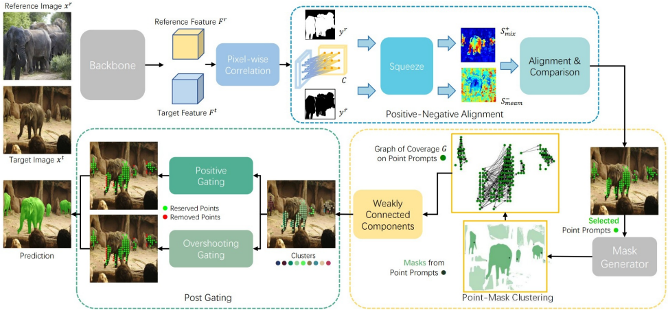
Figure 3.10: Architecture of GFSAM, from A. Zhang et al. (2024).
