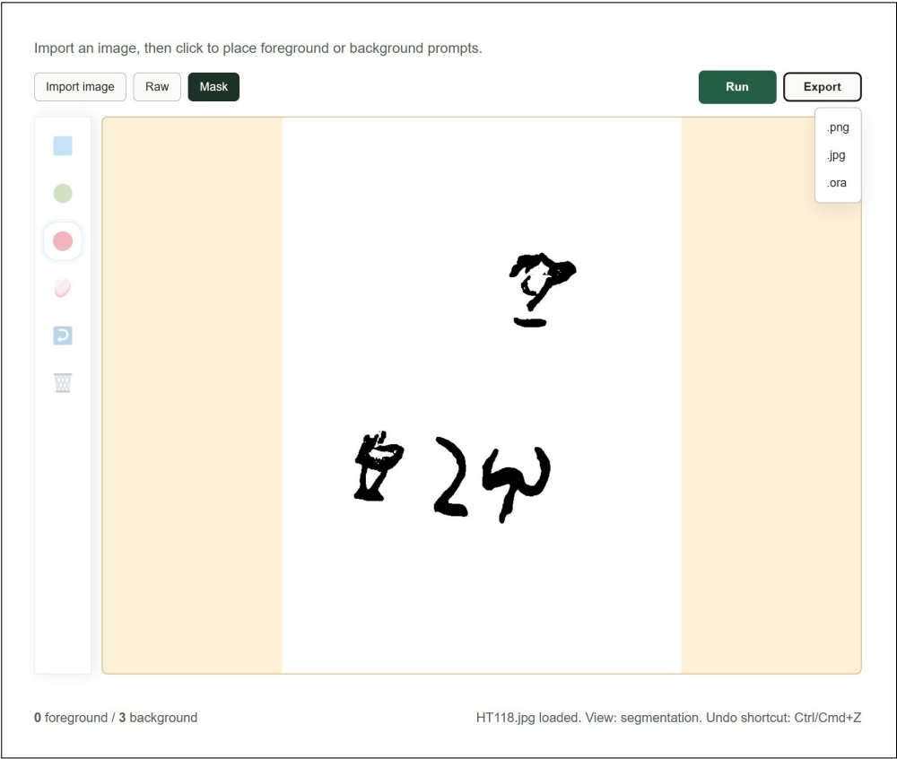
Figure 3.14: In-tool view before export of the mask generated from the prompts placed as seen in Figure 3.13.
