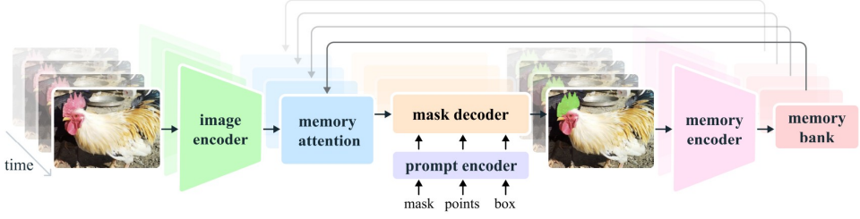
Figure 3.7: Architecture of SAM2, from Ravi et al. (2024).
