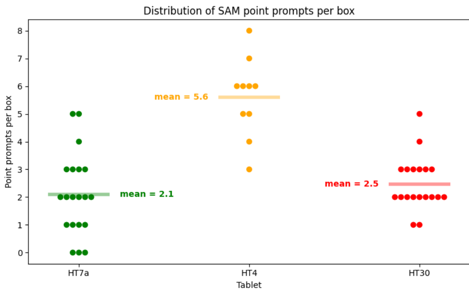
Figure 4.9: Average number of point prompts placed per box prompt for the interactive version of SAM2.
