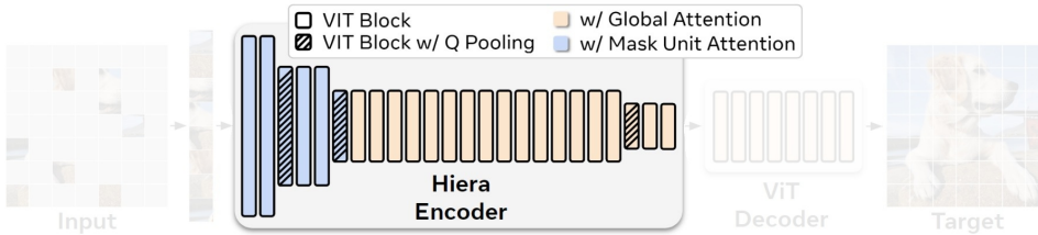
Figure 3.6: Architecture of Hiera, adapted from Ryali et al. (2023).
