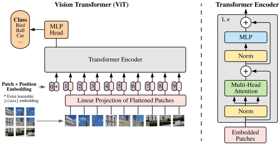
Figure 3.4: Architecture of the ViT, from Dosovitskiy et al. (2021).
