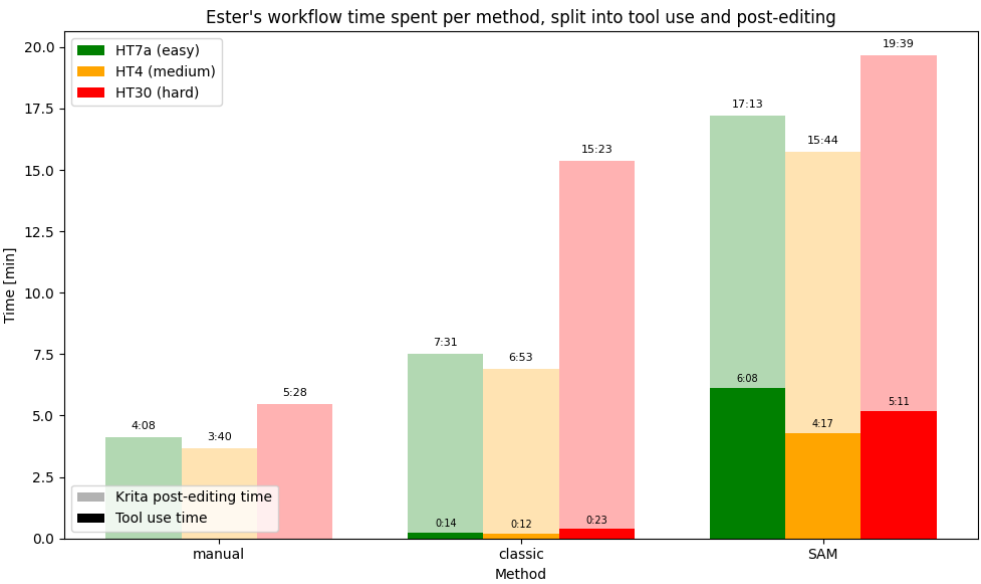
Figure 4.10: Workflow time spent per method, split into phases of tool use (opaque colors) and post-editing in Krita (semi-transparent colors).
