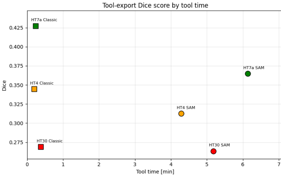
Figure 4.6: Dice scores of the exported masks as a function of tool time, comparing the SAM-based tool to the tool based on the classical baseline.
