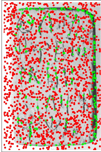
Figure 3.11: A visual example of prompt distribution for SAM with automatic point prompts (SAM+pts), overlaid on HT7a. Green points represent foreground point prompts, while red points represent background point prompts.
