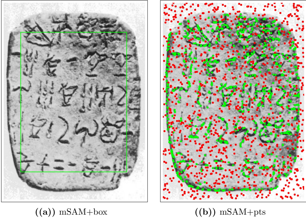
Figure 3.2: A visualization of MobileSAMv2 with automatic box prompts (mSAM+box), and MobileSAMv2 with automatic point prompts (mSAM+pts), overlayed on HT118.
