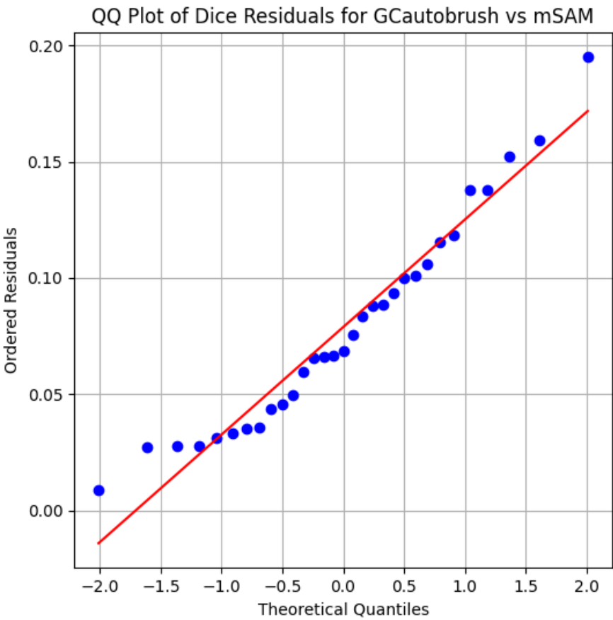
Figure 4.3: QQplot of the residuals of the paired t-test comparing GCautobrush and mSAM. The residuals appear to be approximately normally distributed, which supports the validity of the paired t-test results. Furthermore, the Shapiro-Wilk test for normality on these residuals yields a p-value of 0.16 > \alpha = 0.05 , indicating that we fail to reject the null hypothesis of normality.
