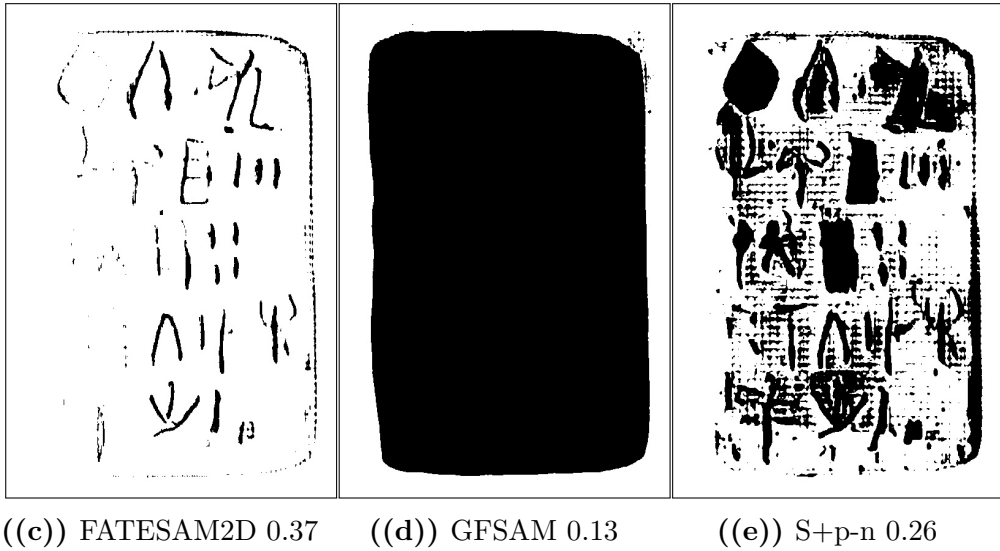
Figure 4.3: Visual comparison of output masks per ICL model and best SAM variant from Section 4.1.1 based on the segmentation of HT7a (easy), shown with Dice scores next to the raw image and ground truth. This is one of the instances where FATESAM2D performed better than the best zero-shot SAM implementation, but due to its tendency of undersegmentation, this was generally not the case.
