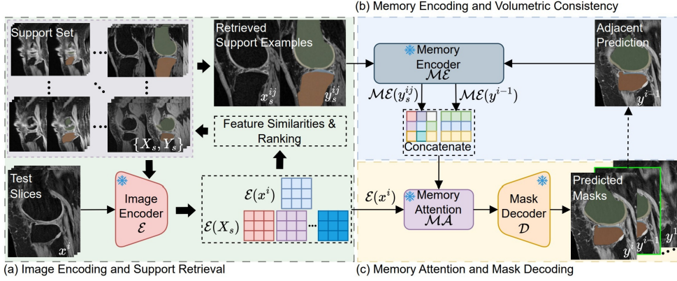
Figure 3.6: Architecture of FATESAM, from He et al. (2025b).
