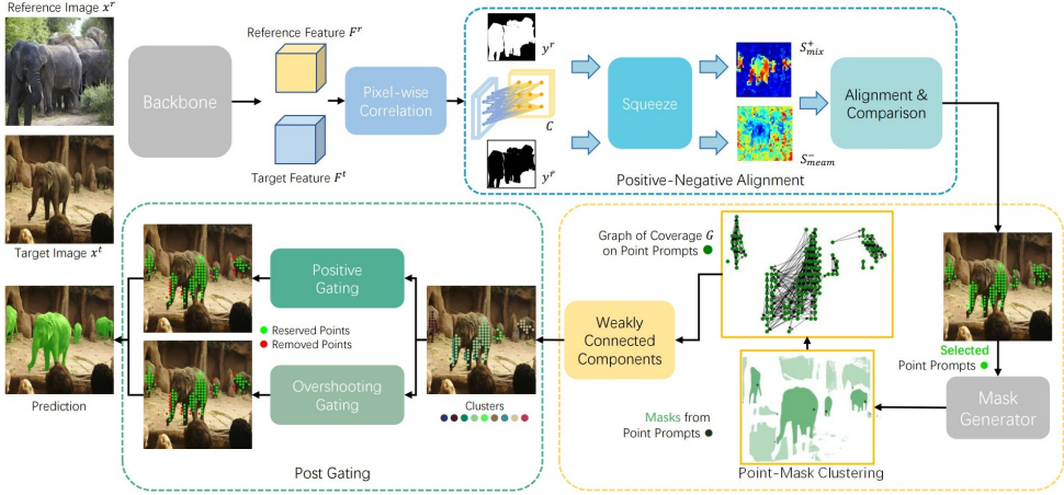
Figure 3.7: Architecture of GFSAM, from A. Zhang et al. (2024).
