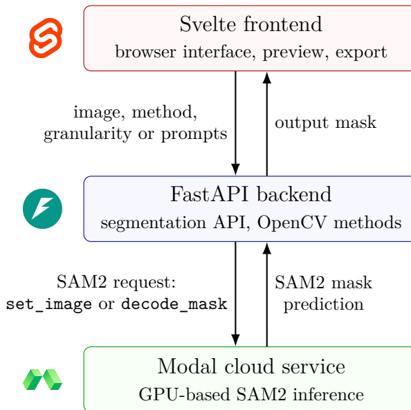
Figure 3.9: Software architecture of the developed segmentation tool, showing the communication between the browser frontend, backend API, and cloud-based SAM2 inference service.
