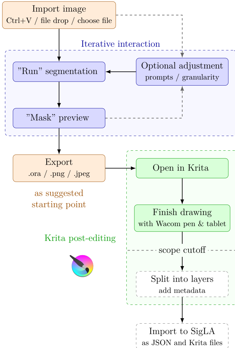
Figure 3.13: User-facing workflow of the developed segmentation tool (in orange, and blue), its iterative interaction (in blue), and its relation to the existing Krita-based annotation workflow (in green). The scope cutoff marks the upper limit of the workflow that the tool was designed to partially automate.
