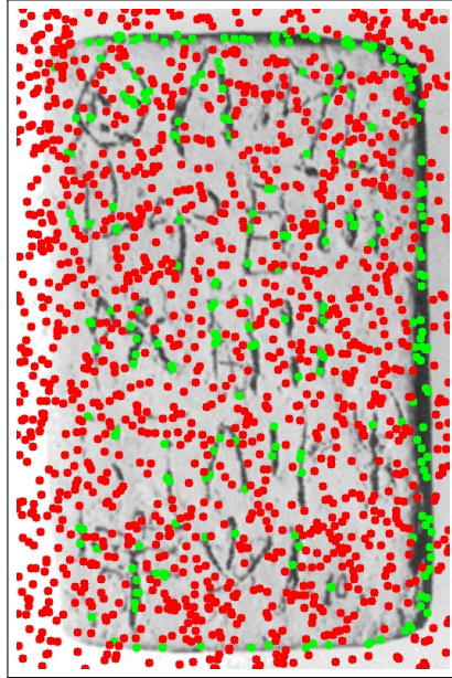
Figure 3.8: A visual example of prompt distribution for SAM with automatic point prompts (SAM+pts), overlaid on HT7a. Green points represent foreground point prompts, while red points represent background point prompts.
