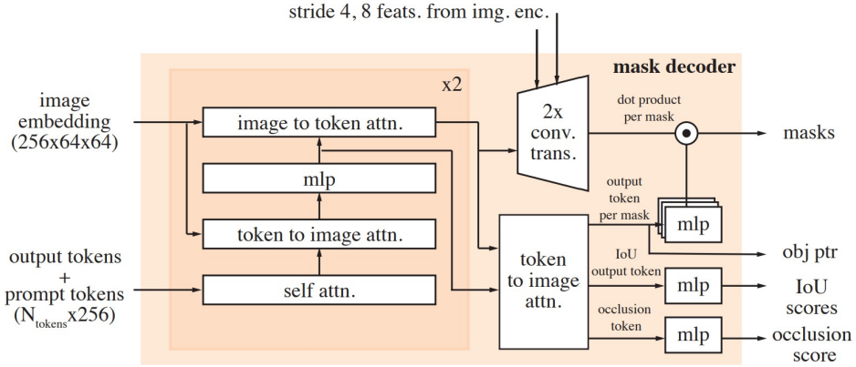
Figure 3.5: Architecture of SAM2’s mask decoder, from Ravi et al. (2024).
