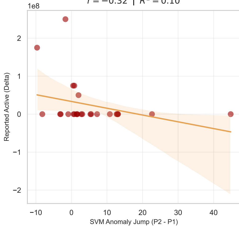
SVM Detection vs. Active
