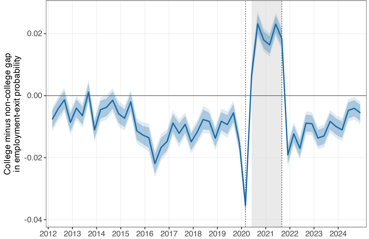
Figure 2: College minus non-college difference in the adjusted probability of employment exit. The dark band is the pointwise 95% interval; the light band is the sup- t simultaneous band over all 52 quarterly contrasts (critical value 2.71).
