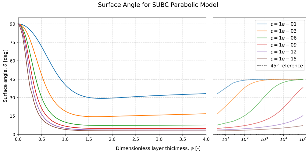
Figure 12: Numerically computed surface angles for a parabolic viscosity profile in the SUBC model. The angles are dependent on the dimensionless parameter \varphi = H/h_{EK} and the background viscosity \epsilon .
