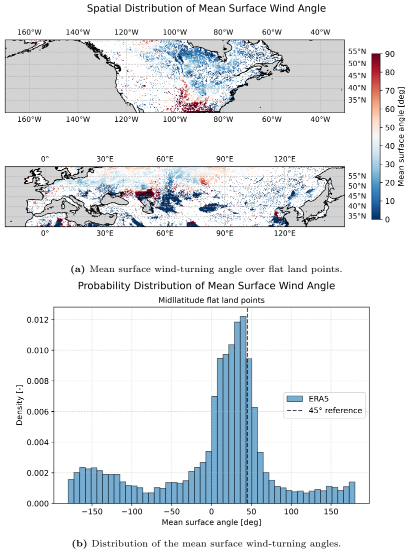
Figure 13: Statistical analysis of the surface wind-turning angles from ERA5 for flat land points located under a jet stream.
