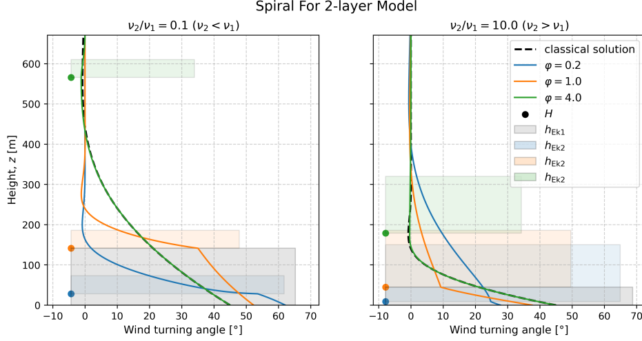
Figure 3: The vertical spiral of the velocities for the two layer model. The angle is dependent on the dimensionless parameter \varphi = H/h_{Ek1} . The classical Ekman solution (when \nu_{const} = \nu_1 ) is shown as a reference.
