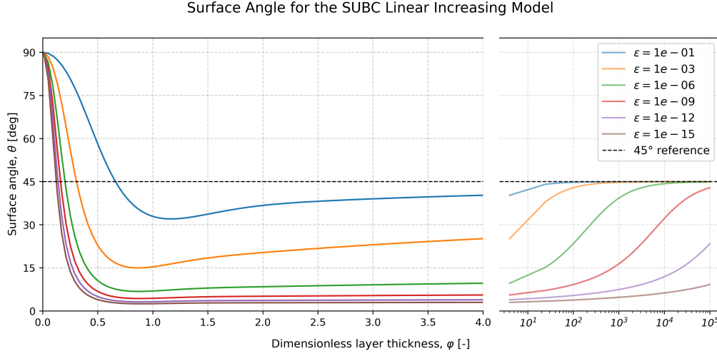
Figure 13: Numerically computed surface angles for linearly increasing. The angles are dependent on the dimensionless parameter \varphi = \tilde{h}_{\text{Ek}}^{-1} and the background viscosity \epsilon .
