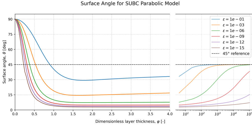
Figure 14: Numerically computed surface angles for a parabolic viscosity profile in the SUBC model. The values are dependent on the dimensionless parameter \varphi = \tilde{h}_{\text{Ek}}^{-1} and the background viscosity \epsilon .
