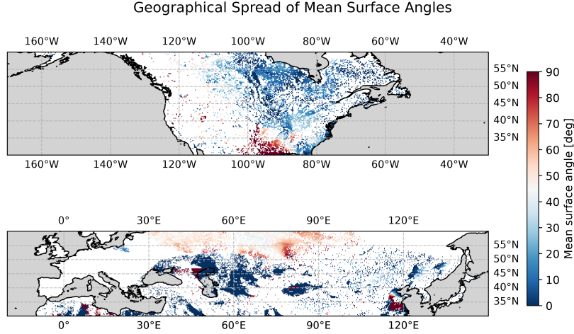
(a) Mean surface wind-turning angle over flat land points from ERA5.
