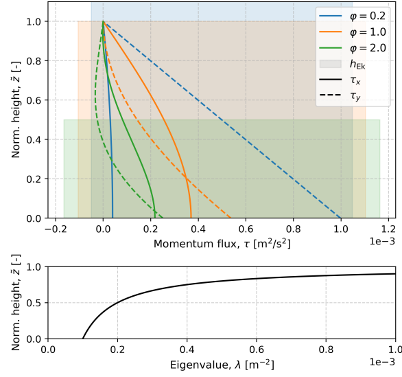
Momentum Flux and Potential for SUBC Linear Decreasing Model
