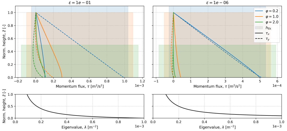
Momentum Flux and Potential for SUBC Linear Increasing Model
