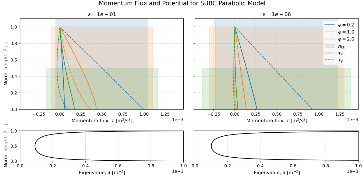
Figure 9: Numerically computed vertical structure for parabolic viscosity. The momentum flux is dependent on the dimensionless parameter \varphi = \tilde{h}_{Ek}^{-1} and the background viscosity \epsilon . The corresponding Ekman heights and eigenvalue are shown with i the figure.
