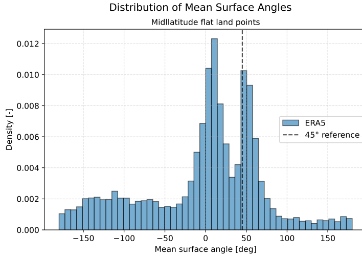
(b) Distribution of the mean surface wind-turning angles.
