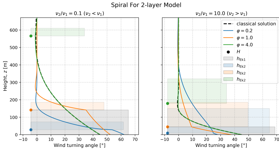
Figure 3: The vertical spiral of the velocities for the two layer model. The angle is dependent on the dimensionless parameter \varphi = H/h_{\text{Ek1}} . The classical Ekman solution (when \nu_{\text{const}} = \nu_1 ) is shown as a reference.
