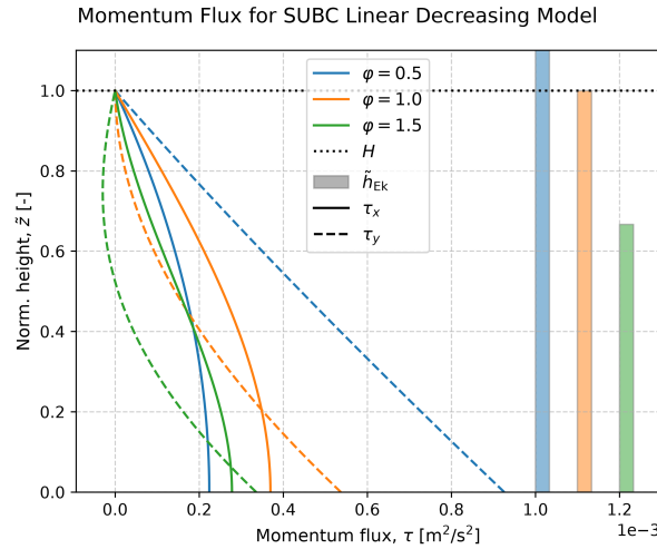
Figure 7: Numerically computed vertical structure for linearly decreasing viscosity. The momentum flux is dependent on the dimensionless parameter \varphi = \tilde{h}_{\text{EK}}^{-1} . The solution assumed a purely zonal geostrophic flow U_g = 10 \text{ m s}^{-1} and a Coriolis parameter of f = 1 \times 10^{-4} \text{ s}^{-1} .
