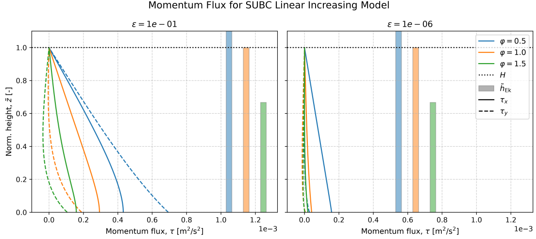
Figure 8: Numerically computed vertical structure for linearly increasing viscosity. The momentum flux is dependent on the dimensionless parameter \varphi = \tilde{h}_{\text{Ek}}^{-1} and the background viscosity \epsilon . The solution assumed a purely zonal geostrophic flow U_g = 10 \text{ m s}^{-1} and a Coriolis parameter of f = 1 \times 10^{-4} \text{ s}^{-1} .
