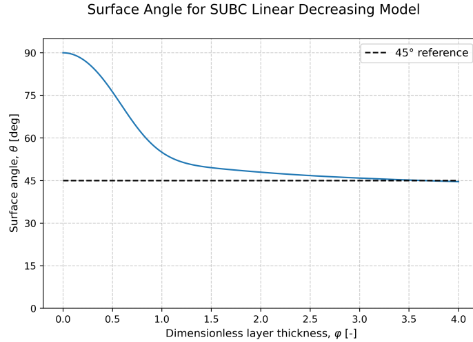
Figure 10: Numerically computed surface angles for decreasing viscosity profiles in the SUBC model. The angle is dependent on the dimensionless parameter \varphi = H/h_{Ek} . The solution assumed a purely zonal geostrophic flow.
