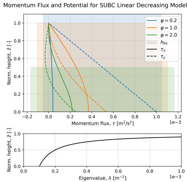
Figure 7: Numerically computed vertical structure for linearly decreasing viscosity. The momentum flux is dependent on the dimensionless parameter \varphi = \tilde{h}_{\text{Ek}}^{-1} . The corresponding Ekman heights and eigenvalue is shown with the shown with the vertical momentum flux. The solution assumed a purely zonal geostrophic flow.
