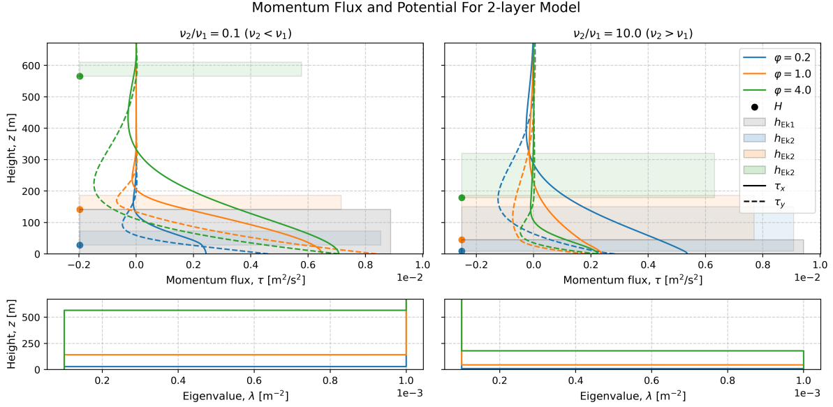
Figure 1: The vertical structure of the momentum flux for the two layer model. The momentum flux is dependent on the dimensionless parameter \varphi = H/h_{Ek1} and the ratio of the viscosities. The corresponding Ekman heights and eigenvalue is shown with the vertical momentum flux. The solution assumed a purely zonal geostrophic flow and a Coriolis parameter of f = 1 \times 10^{-4} \text{ s}^{-1} .
