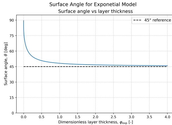
Figure 2: Surface angle for the exponentially decaying viscosity model as a function of the dimensionless parameter \varphi = H/h_{\text{Ek}} . The solution assumed a purely zonal geostrophic flow.
