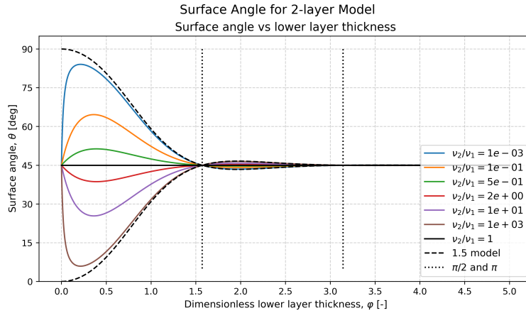
Figure 1: The surface angle as a function of the dimensionless layer thickness \varphi = H/h_{\text{Ek}1} for the two-layer viscosity model. Different coloured curves correspond to different layer viscosity ratios. The classical Ekman angle of 45^\circ is shown as a reference.
