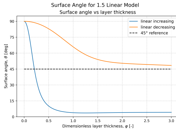
Figure 3: Numerically computed surface angles for linearly increasing and decreasing viscosity profiles in the 1.5-layer model. The angle is dependent on the dimensionless parameter \varphi = H/E_K .
