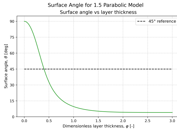
Figure 4: Numerically computed surface angles for a parabolic viscosity profile in the 1.5-layer model. The angle is dependent on the dimensionless parameter \varphi = H/E_K .
