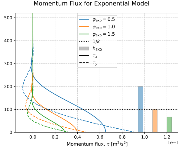
Figure 5: The vertical structure of the momentum flux for exponentially decreasing viscosity together with the corresponding Ekman height and inverse decay rate. The momentum flux is dependent on the dimensionless parameter \varphi_{exp} = 1/k h_{Ek0} . The solution assumed a purely zonal geostrophic flow U_g = 10 \text{ m s}^{-1} , a Coriolis parameter of f = 1 \times 10^{-4} \text{ s}^{-1} , a decay rate of k = 1 \times 10^{-2} \text{ m}^{-1} and initial viscosities of \nu_0 = 12.5 \text{ m}^2 \text{ s}^{-1} , \nu_0 = 0.5 \text{ m}^2 \text{ s}^{-1} and \nu_0 = 0.03125 \text{ m}^2 \text{ s}^{-1} .
