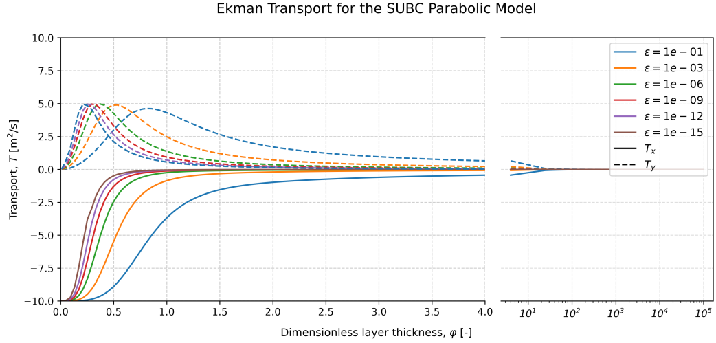
Figure 17: Numerically computed Ekman transport for a parabolic viscosity profile in the SUBC model. The angles are dependent on the dimensionless parameter \varphi = H/h_{\text{EK}} and the background viscosity \epsilon .
