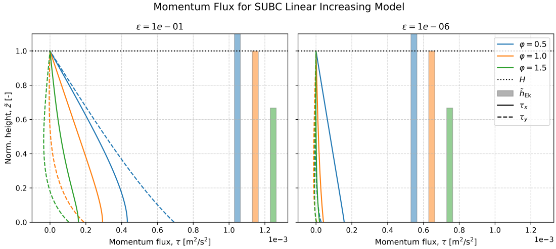
Figure 10: Numerically computed vertical structure for linearly increasing viscosity. The momentum flux is dependent on the dimensionless parameter \varphi = \tilde{h}_{\text{Ek}}^{-1} and the background viscosity \epsilon . The solution assumed a purely zonal geostrophic flow U_g = 10 \text{ m s}^{-1} and a Coriolis parameter of f = 1 \times 10^{-4} \text{ s}^{-1} .
