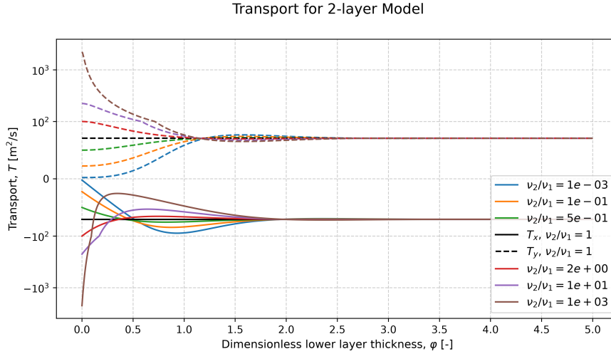
Figure 4: The total transport as a function of the dimensionless layer thickness \varphi = H/h_{\text{Ek1}} for the two-layer model. Different coloured curves correspond to different layer viscosity ratios. The solution assumed \nu_1 = 0.01 \text{ m}^2 \text{ s}^{-1} .
