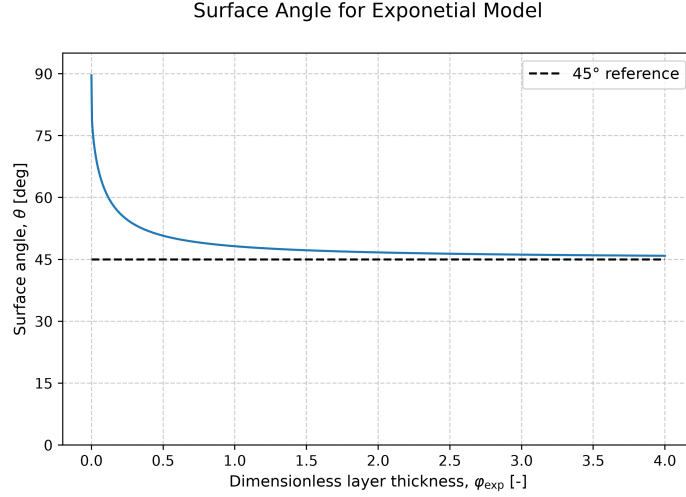
Figure 6: Surface angle for the exponentially decaying viscosity model as a function of the dimensionless parameter \varphi_{\text{exp}} = H/h_{\text{Ek}0} . The same parameters as in Figure 5 was used.
