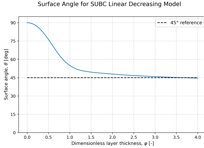
Figure 12: Numerically computed surface angles for decreasing viscosity profiles in the SUBC model. The angles are dependent on the dimensionless parameter \varphi = H/h_{\text{Ek}} .
