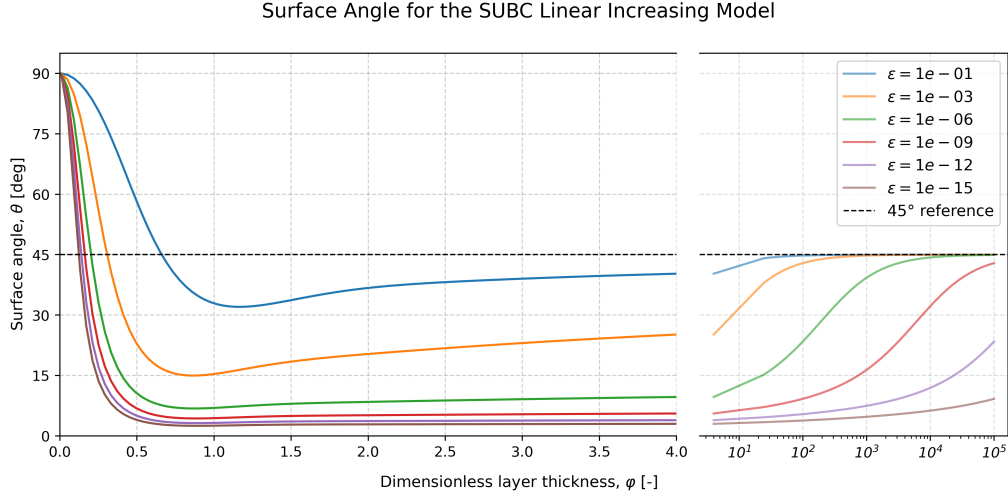
Figure 13: Numerically computed surface angles for linearly increasing. The angles are dependent on the dimensionless parameter \varphi = H/h_{EK} and the background viscosity \epsilon .
