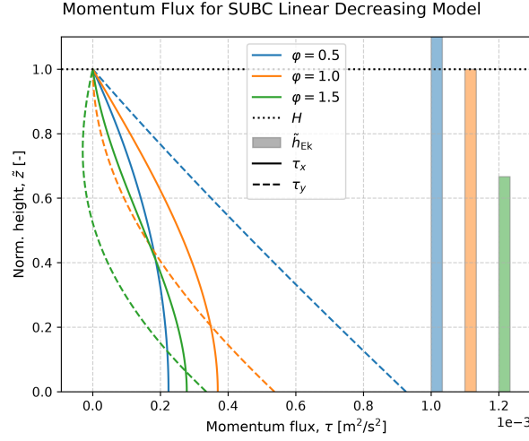
Figure 9: Numerically computed vertical structure for linearly decreasing viscosity. The momentum flux is dependent on the dimensionless parameter \varphi = \tilde{h}_{\text{Ek}}^{-1} . The solution assumed a purely zonal geostrophic flow U_g = 10 \text{ m s}^{-1} and a Coriolis parameter of f = 1 \times 10^{-4} \text{ s}^{-1} .
