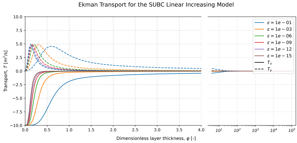
Figure 16: Numerically computed Ekman transport for a linear increasing viscosity profile in the SUBC model. The values are dependent on the dimensionless parameter \varphi = H/h_{EK} and the background viscosity \epsilon .
