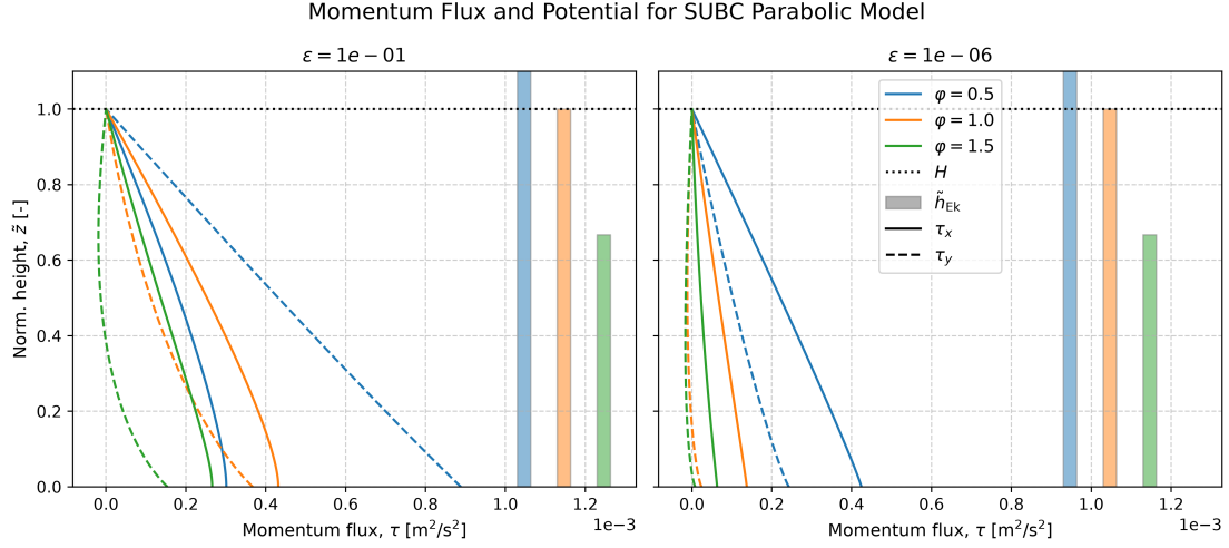
Figure 11: Numerically computed vertical structure for parabolic viscosity. The momentum flux is dependent on the dimensionless parameter \varphi = \tilde{h}_{\text{Ek}}^{-1} and the background viscosity \epsilon . The solution assumed a purely zonal geostrophic flow U_g = 10 \text{ m s}^{-1} and a Coriolis parameter of f = 1 \times 10^{-4} \text{ s}^{-1} .
