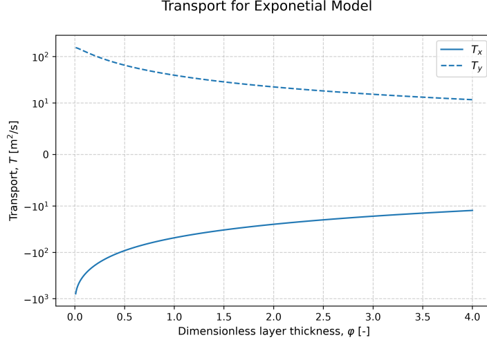
Figure 8: The total transport as a function of the dimensionless layer thickness \varphi_{\text{exp}} = 1/k h_{\text{Ek}0} for the exponential model. The solution assumed k = 0.1 \text{ m}^{-1} .
