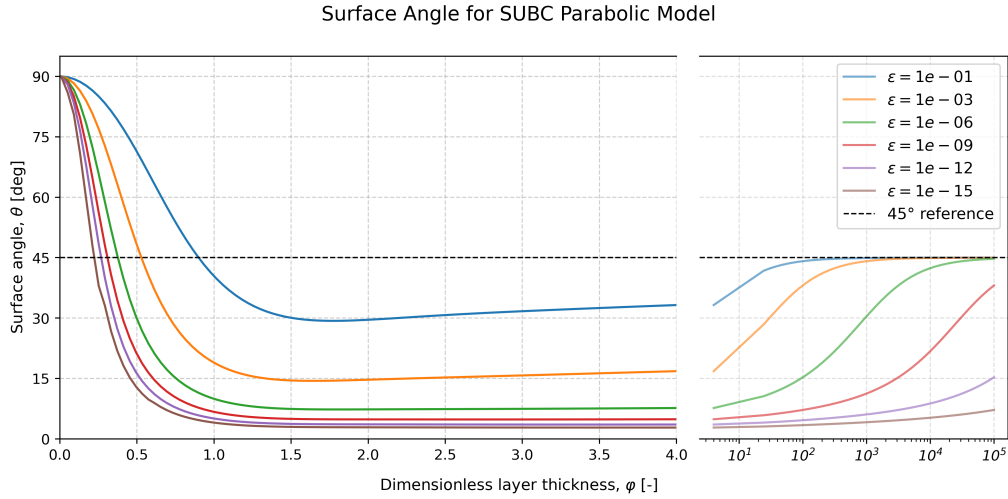
Figure 14: Numerically computed surface angles for a parabolic viscosity profile in the SUBC model. The values are dependent on the dimensionless parameter \varphi = H/h_{EK} and the background viscosity \epsilon .
