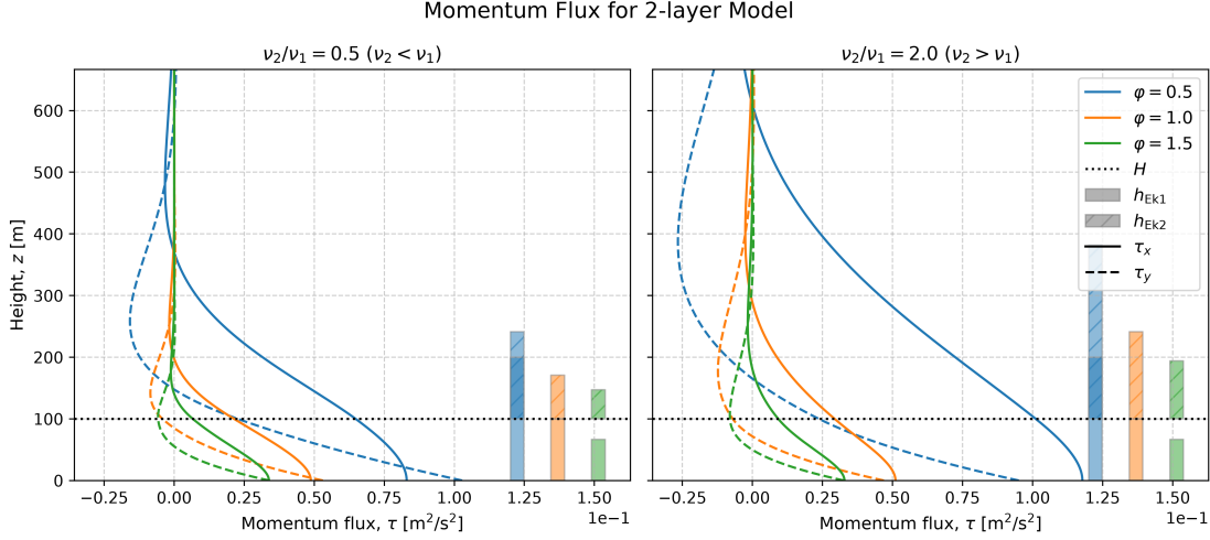
Figure 1: The vertical structure of the momentum flux for the two layer model. The momentum flux is dependent on the dimensionless parameter \varphi = H/h_{\text{Ek1}} and the ratio of the viscosities. The corresponding Ekman heights and interface are shown with the vertical momentum flux. The solution assumed a purely zonal geostrophic flow U_g = 10 \text{ m s}^{-1} , a Coriolis parameter of f = 1 \times 10^{-4} \text{ s}^{-1} and an intersection height of H = 100 \text{ m} . The lower viscosities, derived from H and \varphi , are \nu_1 = 2 \text{ m}^2/\text{s} , \nu_1 = 5 \times 10^{-1} \text{ m}^2/\text{s} , and \nu_1 = 2.22 \times 10^{-1} \text{ m}^2/\text{s} in both figures. In the left figure, \nu_2 used half the value of the lower viscosities, and in the right figure, it used double of that value.
