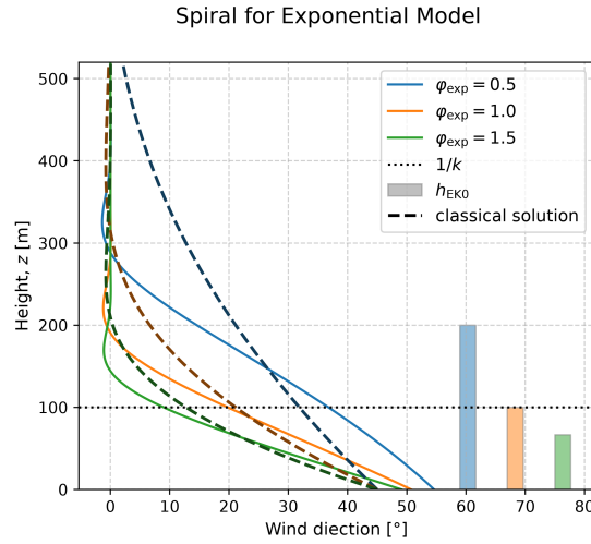
Figure 7: The vertical spiral for the exponentially decreasing viscosity model together with the Ekman height and the inverse decay rate. The wind direction is dependent on the dimensionless parameter \varphi_{\text{exp}} = 1/k h_{\text{Ek}0} . The classical Ekman solution (for \nu_0 ) is shown as a reference. The parameters had the same values as in Figure 5.
