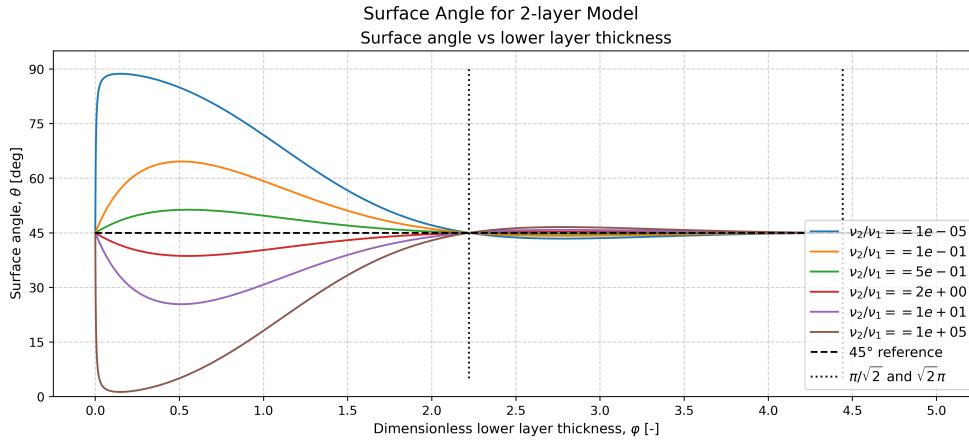
Figure 1: The surface angle as a function of the dimensionless layer thickness \varphi = H/h_{EK1} for the two-layer viscosity model. Different coloured curves correspond to different layer viscosity ratios. The classical Ekman angle of 45° is shown as a reference.
