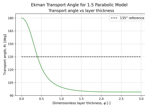
Figure 8: Numerically computed transport angles for a parabolic viscosity profile in the 1.5-layer model. The angle is dependent on the dimensionless parameter \varphi = H/h_{EK} . The solution assumed a purely zonal geostrophic flow.
