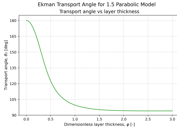
Figure 6: Numerically computed transport angles for a parabolic viscosity profile in the 1.5-layer model. The angle is dependent on the dimensionless parameter \varphi = H/h_{EK} . The solution assumed a purely zonal geostrophic flow.
