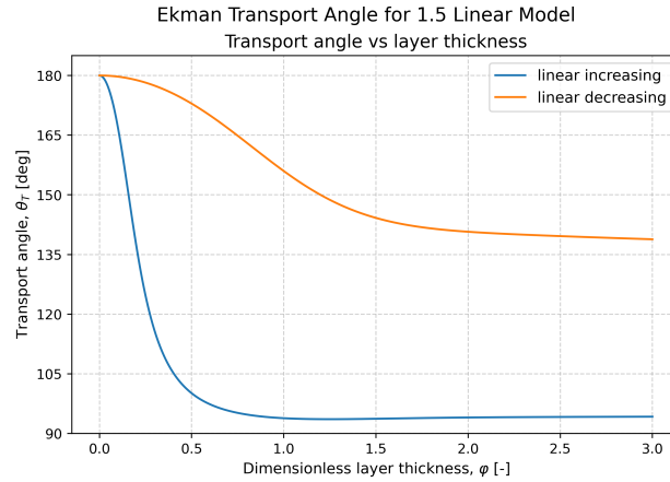
Figure 5: Numerically computed transport angles for linearly increasing and decreasing viscosity profiles in the 1.5-layer model. The angle is dependent on the dimensionless parameter \varphi = H/h_{EK} . The solution assumed a purely zonal geostrophic flow.
