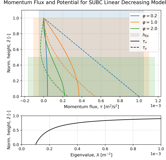
Figure 5: Numerically computed vertical structure for linearly decreasing viscosity. The momentum flux is dependent on the dimensionless parameter \varphi = \tilde{h}_{\text{Ek}}^{-1} . The corresponding Ekman heights and eigenvalue is shown with the shown with the vertical momentum flux. The solution assumed a purely zonal geostrophic flow.
