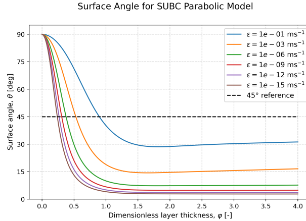
Figure 10: Numerically computed surface angles for a parabolic viscosity profile in the SUBC model. The angle is dependent on the dimensionless parameter \varphi = H/h_{EK} and the background viscosity \epsilon . The solution assumed a purely zonal geostrophic flow.
