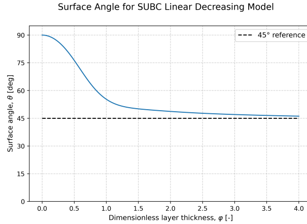
Figure 8: Numerically computed surface angles for decreasing viscosity profiles in the SUBC model. The angle is dependent on the dimensionless parameter \varphi = H/h_{\text{Ek}} . The solution assumed a purely zonal geostrophic flow.
