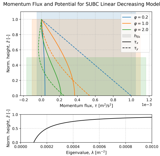
Figure 5: Numerically computed vertical structure for linearly decreasing viscosity. The momentum flux is dependent on the dimensionless parameter \varphi = H/h_{\text{EK}} = 1/h_{\text{EK}} . The corresponding Ekman heights and eigenvalue is shown with the shown with the vertical momentum flux. The solution assumed a purely zonal geostrophic flow.
