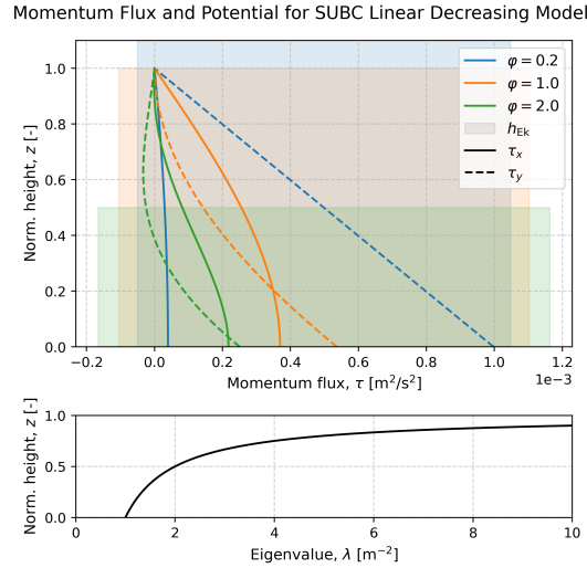
Figure 5: Numerically computed vertical structure for linearly decreasing viscosity. The momentum flux is dependent on the dimensionless parameter \varphi = H/h_{Ek} = 1/\tilde{\nu}_{Ek} . The corresponding Ekman heights and viscosity potential is shown with the vertical momentum flux. The solution assumed a purely zonal geostrophic flow.
