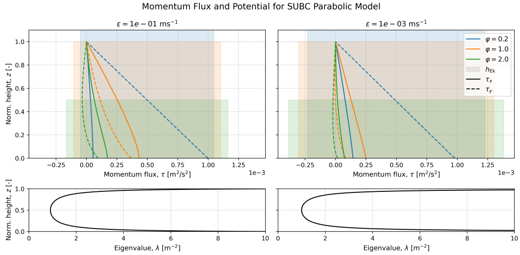
Figure 7: Numerically computed vertical structure for parabolic viscosity. The momentum flux is dependent on the dimensionless parameter \varphi = H/h_{Ek} = 1/\tilde{h}_{Ek} and the background viscosity \epsilon . The corresponding Ekman heights and viscosity potential is shown with the shown with the vertical momentum flux. The solution assumed a purely zonal geostrophic flow.
