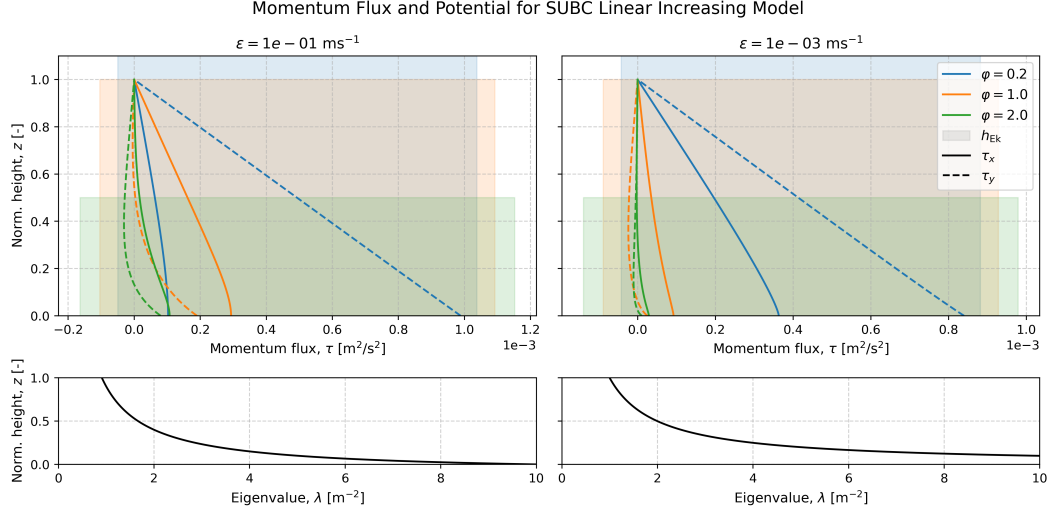
Figure 6: Numerically computed vertical structure for linearly increasing viscosity. The momentum flux is dependent on the dimensionless parameter \varphi = H/h_{Ek} = 1/\tilde{h}_{Ek} and the background viscosity \epsilon . The corresponding Ekman heights and viscosity potential is shown with the shown with the vertical momentum flux. The solution assumed a purely zonal geostrophic flow.
