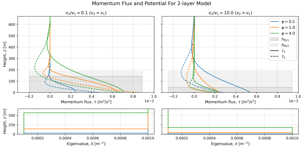
Figure 1: The vertical structure of the momentum flux for a two layer viscosity. The momentum flux is dependent on the dimensionless parameter \varphi = H/h_{\text{Ek1}} and the ratio of the viscosities. The corresponding Ekman heights and viscosity potential is shown with the shown with the vertical momentum flux. The solution assumed a purely zonal geostrophic flow.
