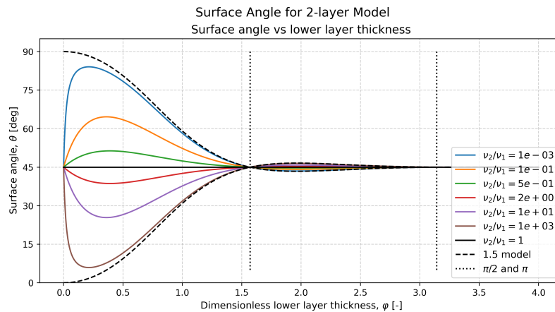
Figure 1: The surface angle as a function of the dimensionless layer thickness \varphi = H/h_{Ek1} for the two-layer viscosity model. Different coloured curves correspond to different layer viscosity ratios. The classical Ekman angle of 45^\circ is shown as a reference.
