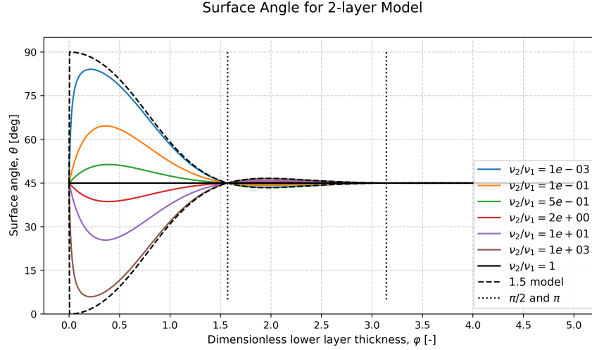
Figure 2: The surface angle as a function of the dimensionless layer thickness \varphi = H/h_{\text{Ek1}} for the two-layer viscosity model. Different coloured curves correspond to different layer viscosity ratios. The classical Ekman angle of 45^\circ is shown as a reference.
