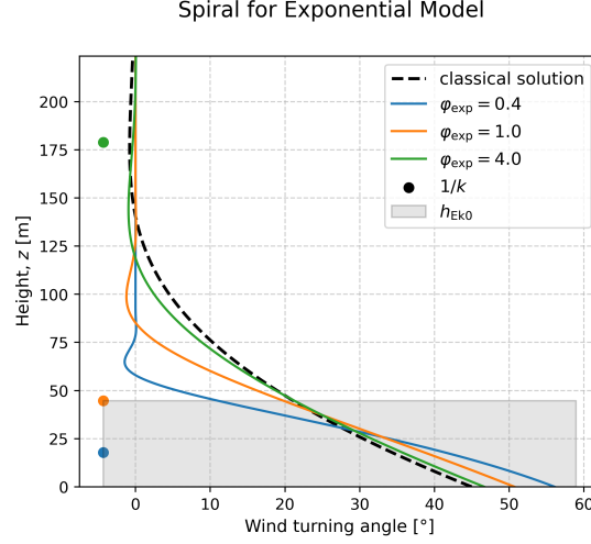
Figure 6: The vertical spiral of the velocities for exponentially decreasing viscosity. The angle is dependent on the dimensionless parameter \varphi_{\text{exp}} = 1/k h_{\text{Ek}0} . The classical Ekman solution (for \nu_0 ) is also shown. The solution assumed a purely zonal geostrophic flow and a Coriolis parameter of f = 1 \times 10^{-4} \text{ s}^{-1}
