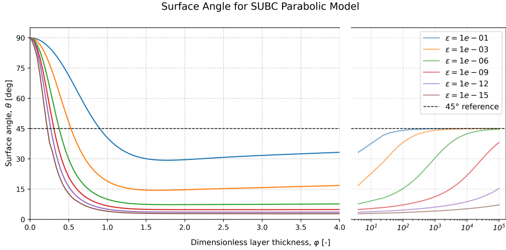
Figure 12: Numerically computed surface angles for a parabolic viscosity profile in the SUBC model. The angle is dependent on the dimensionless parameter \varphi = H/h_{EK} and the background viscosity \epsilon . The solution assumed a purely zonal geostrophic flow.
