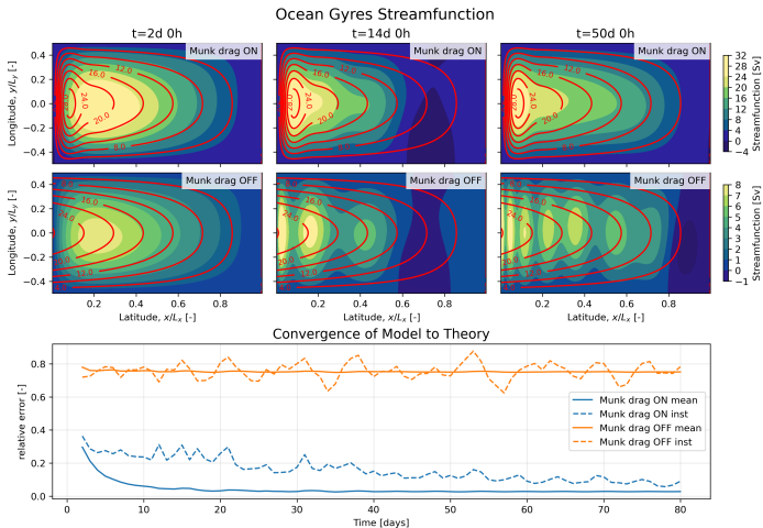
Figure: Streamfunction for the Laplace-viscous \beta -plane configuration.
