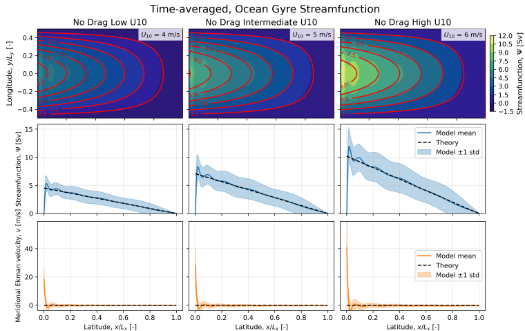
Figure: Streamfunction for the no-drag \beta -plane configuration.
