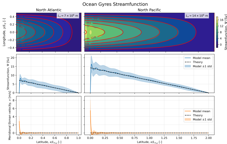
Figure: Streamfunction for the no-drag \beta -plane configuration with varying domain size.
