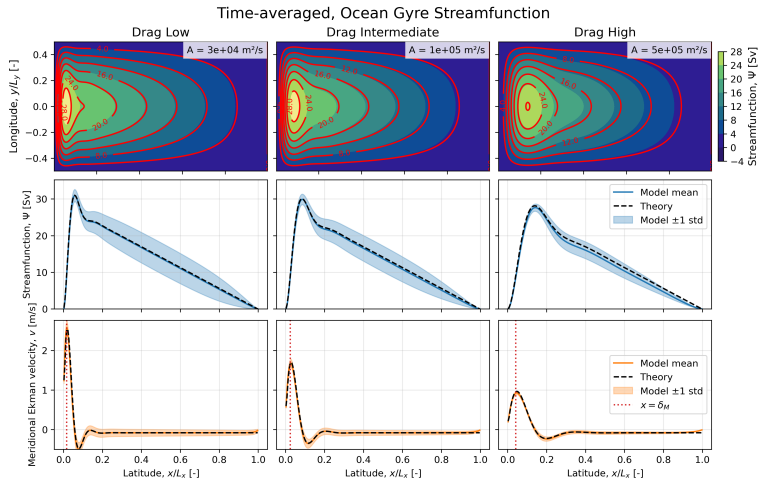
Figure: Streamfunction for the Laplace-viscous \beta -plane configuration.
