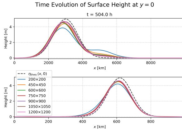
Figure 6: This figure shows the zonal propagation of the Kelvin waves in the two oceans for a bunch of different grid sizes.
