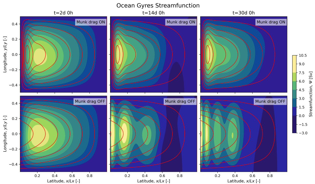
Figure 6: This figure shows the effect of the Munk friction, compared to the Sverdrup theory without friction. This is seen for different time-steps, to highlight the difference in steady state solutions. The Munk theory displays a proper convergence, whereas the Sverdrup does not converge to a steady state solution. The contours show the model result, while the solid red lines showcases the Munk and Sverdrup theory respectively.
