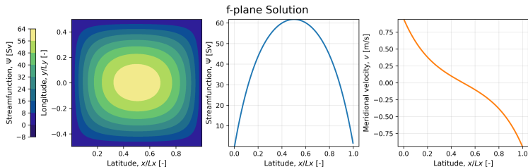
Figure: Streamfunction for the no-drag f -plane configuration. The circulation remains symmetric with no \beta -effect and without western intensification.
