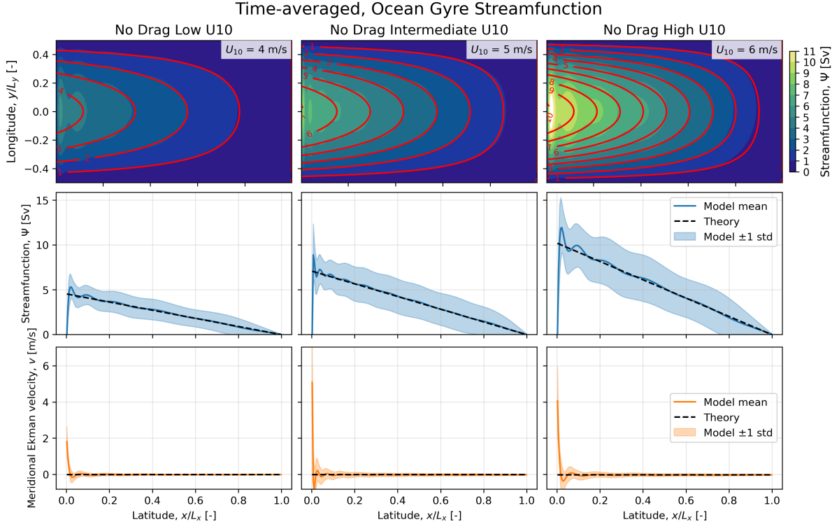
Figure 2: Comparison of streamfunction fields for different ten meter winds. The contours show the model result, while the solid red lines showcase the Sverdrup theory. The cross-sections of the streamfunction is at the center of the domain. The meridional wind velocity has been transformed into an Ekman-layer velocity, by assuming an Ekman depth of \delta_{EK} = 50 m. The meridional velocity is thus the corresponding mass flux as if the domain is at rest and only the Ekman layer is moving. The time averaging was done between two days and eighty days.
