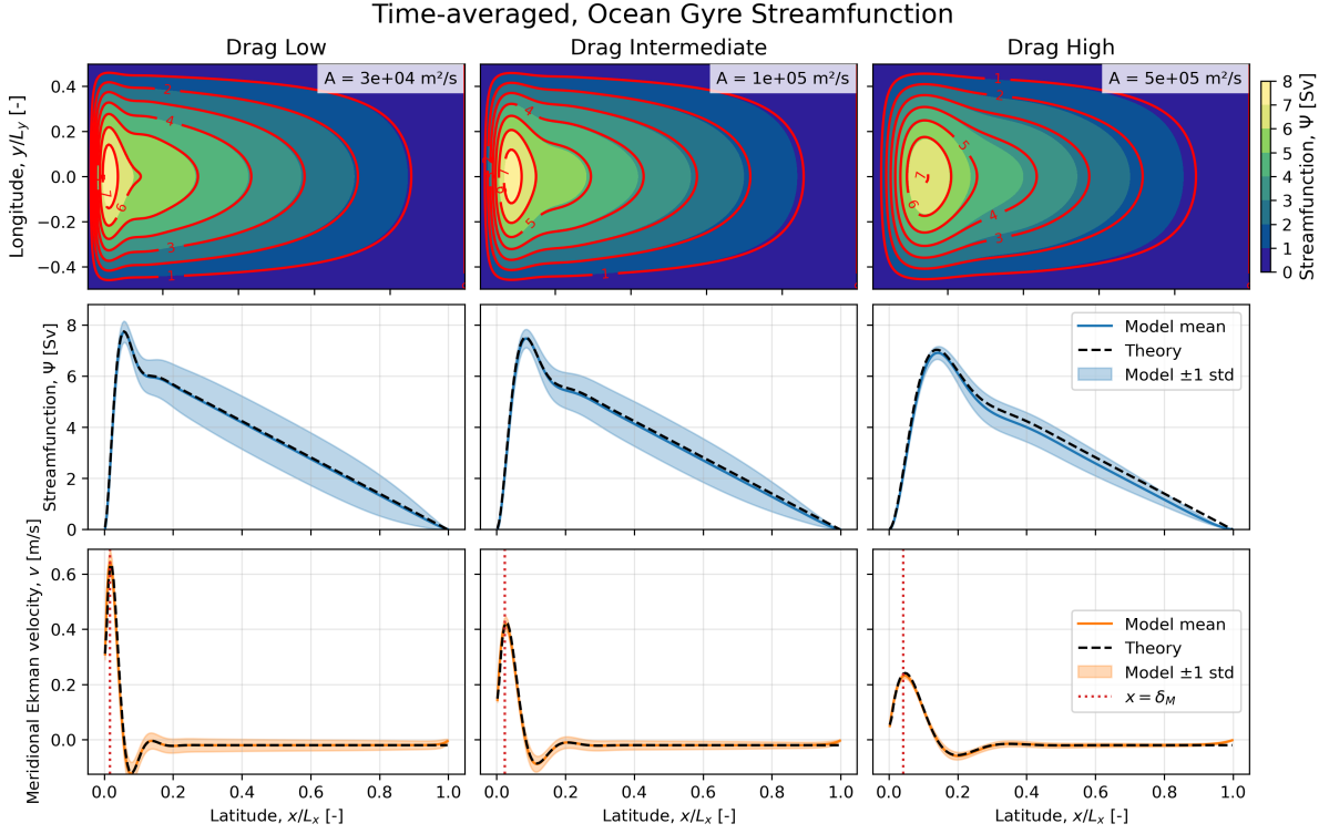
Figure 4: Streamfunction fields for different values of the meridional viscosity coefficient A , compared to Munk theory. The contours show the model result, while the solid red lines showcase the theory. The resolution of the Munk depth is \frac{\delta_M}{\Delta x} = [3.8, 4.9, 8.4] , from left to right in the figure. The center domain zonal cross-sections show solid lines for the numerical model, while dashed lines represent Munk theory. The meridional wind velocity has again been transformed into an Ekman-layer velocity (as explained in Figure 2). The time-averaging was done between two days and eighty days.
