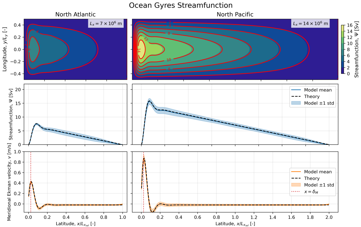
Figure 5: Streamfunction for the viscosity \beta -plane configuration with varying domain size. The contours show the model result, while the solid red lines showcase the Munk theory. In the center domain cross-section, solid lines show the numerical model results, while dashed lines show theory. The meridional wind velocity has been transformed into an Ekman-layer velocity (as explained in Figure 2). The time averaging was done between two days and eighty days.
