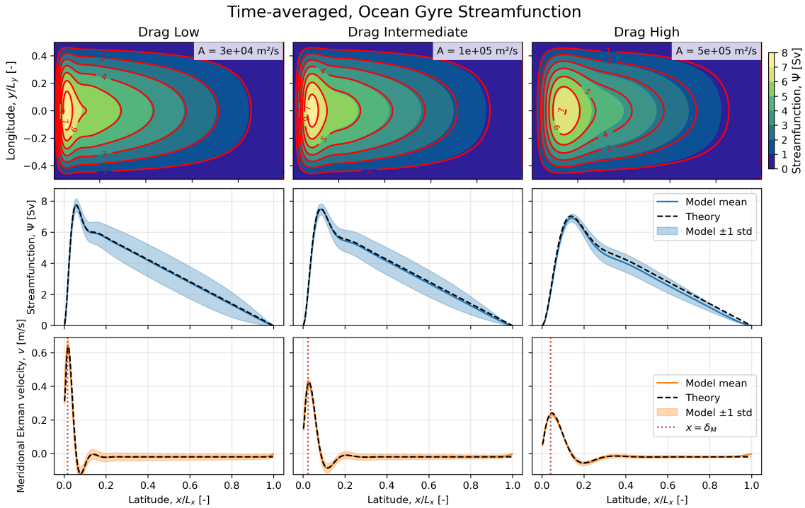
Figure 5: Streamfunction fields for different values of the meridional viscosity coefficient A , compared to Munk theory. The contours show the model result, while the solid red lines showcases the theory. The resolution of the Munk depth is \frac{\delta_M}{\Delta x} = [3.8, 4.9, 8.4] , from left to right in the figure. The center domain zonal cross-sections show solid lines for the numerical model, while dashed lines represent Munk theory. The meridional wind velocity has again been transformed into an Ekman-layer velocity, by assuming an Ekman depth of \delta_{EK} = 50 m. The meridional velocity is thus the corresponding mass flux as if the domain is at rest and only the Ekman layer is moving. The time-averaging was done between two days and two weeks.
