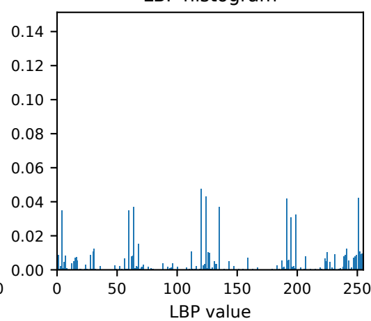
LBP histogram
