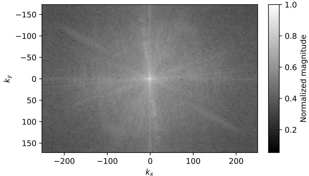
2D DFT
