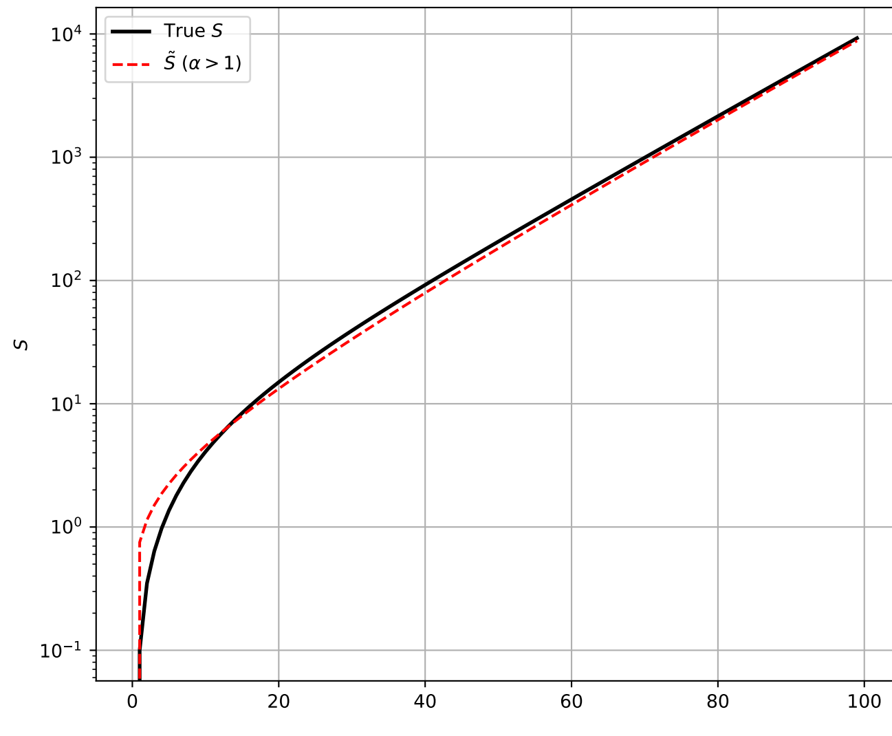
S and \tilde{S} vs. N for \alpha = 1.5
