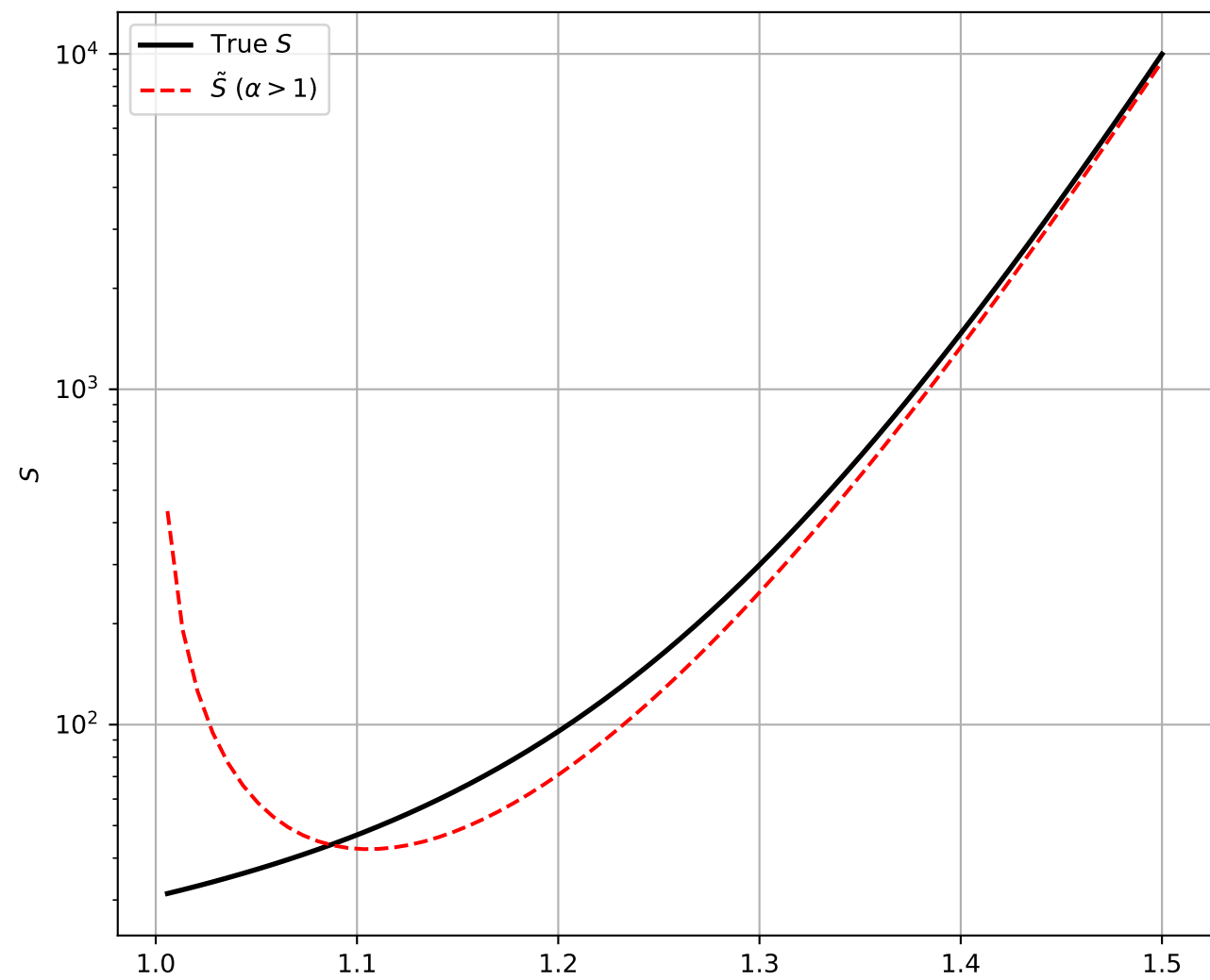
True S and \tilde{S} for \alpha > 1
