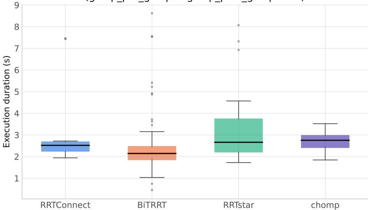
Trajectory execution duration by planner (grasp_pre_grasp + grasp_post_grasp calls)
