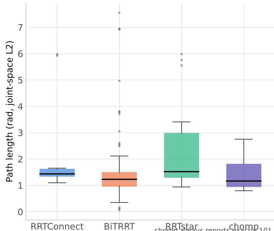
Path length by planner
