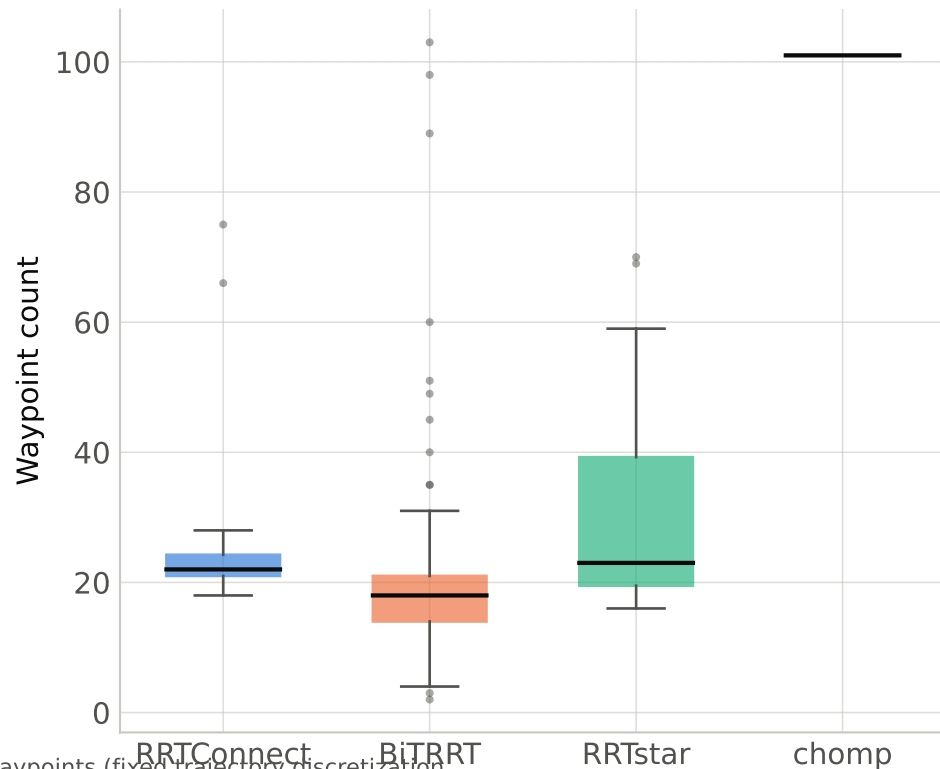
Waypoint count by planner
