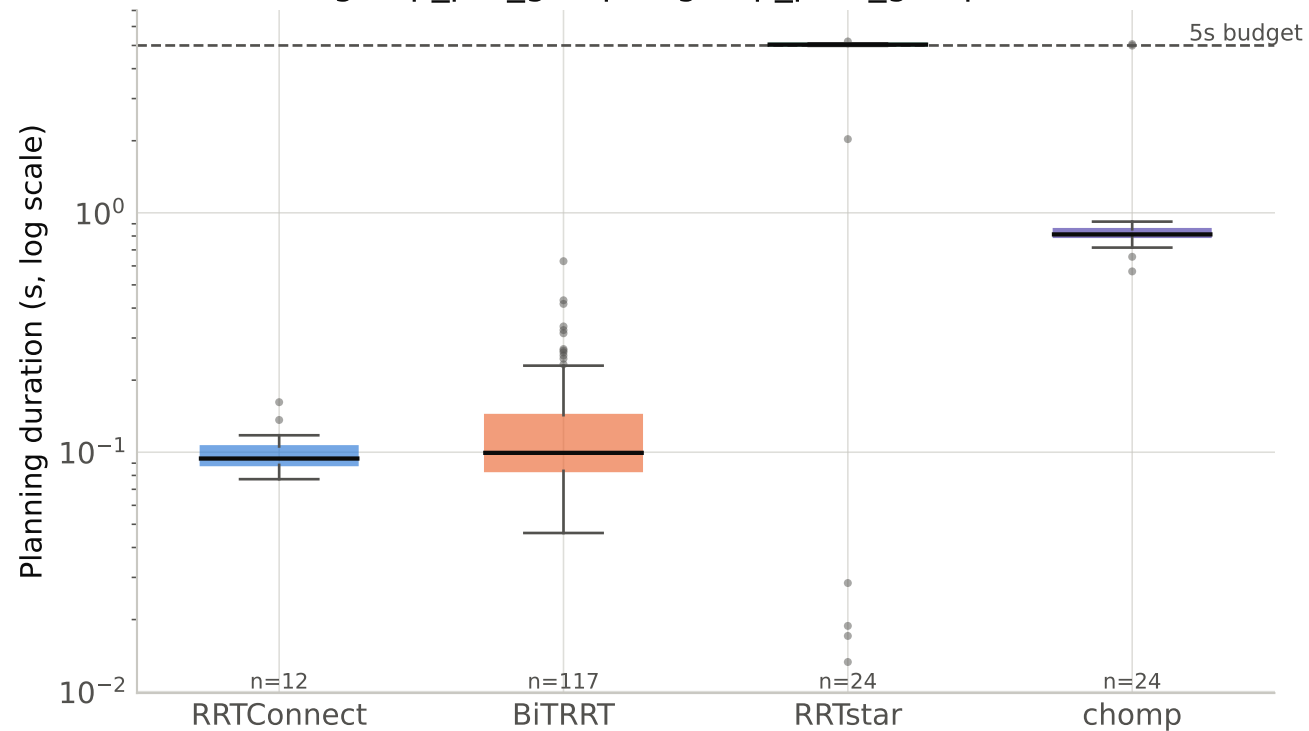
Planning duration by planner (grasp_pre_grasp + grasp_post_grasp calls)
