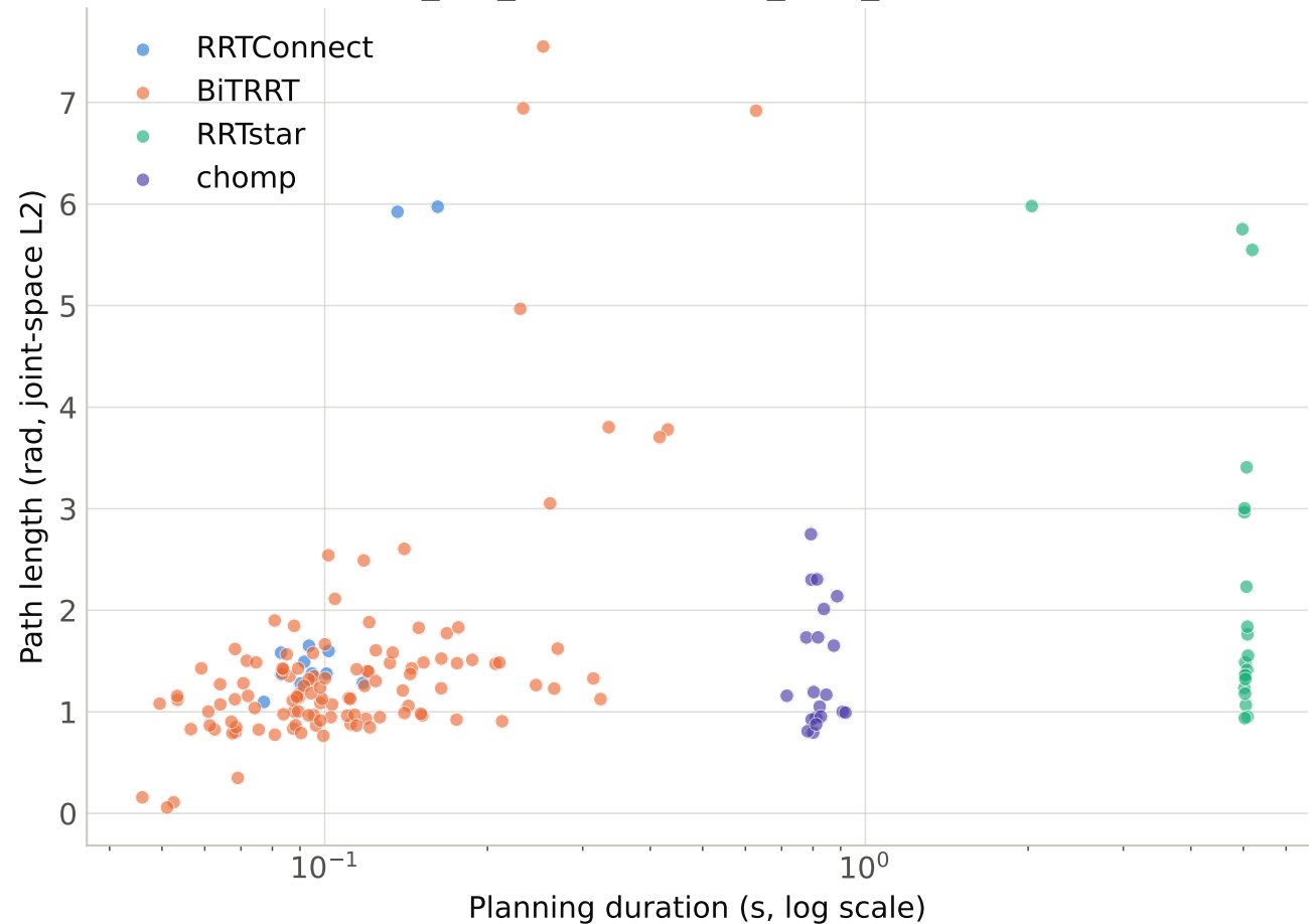
Planning-time / path-quality trade-off (grasp_pre_grasp + grasp_post_grasp calls)
