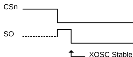
Figure 26: Power-On Reset
