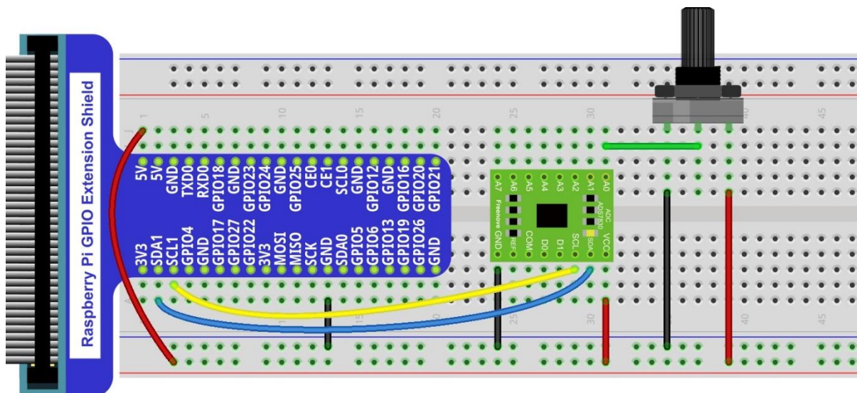
Hardware connection
