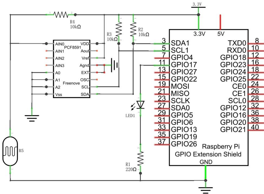
Hardware connection
