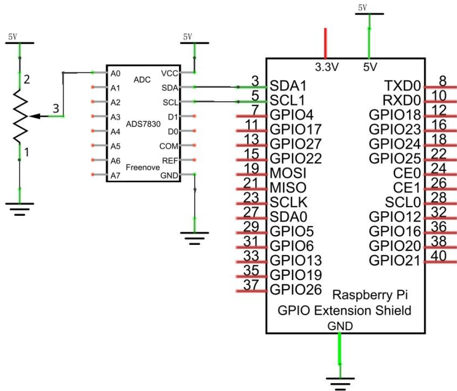
Hardware connection
