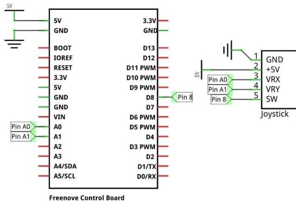
Freenove Control Board
