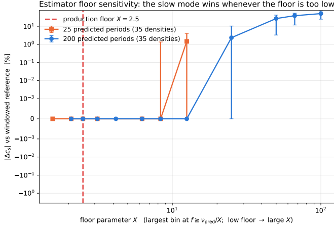
Fig. 3. Floor sensitivity. Median |\Delta c_s| against the windowed reference over all 35 densities, with the 16–84% spread as the error bar, versus the floor parameter X (the floor is \nu_{\text{pred}}/X , so a large X is a low floor). The collapse at large X is the slow mode of Fig. 2 winning the periodogram; it is worse at 200 periods, where the wander has more bins below the resonance. At the production value X = 2.5 the estimator reproduces the windowed reference exactly at both record lengths.
