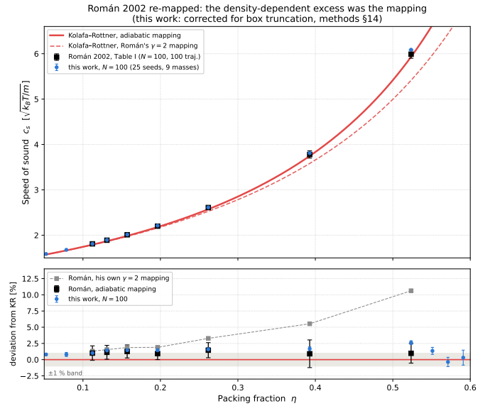
Fig. 11. Román et al. re-mapped. Solid red, Kolafa–Rottner through (1); dashed red, the same equation of state through their \gamma = 2 mapping; black squares, their Table I with their error bars; blue, this work at N = 100 . Lower panel: deviation from Kolafa–Rottner.
