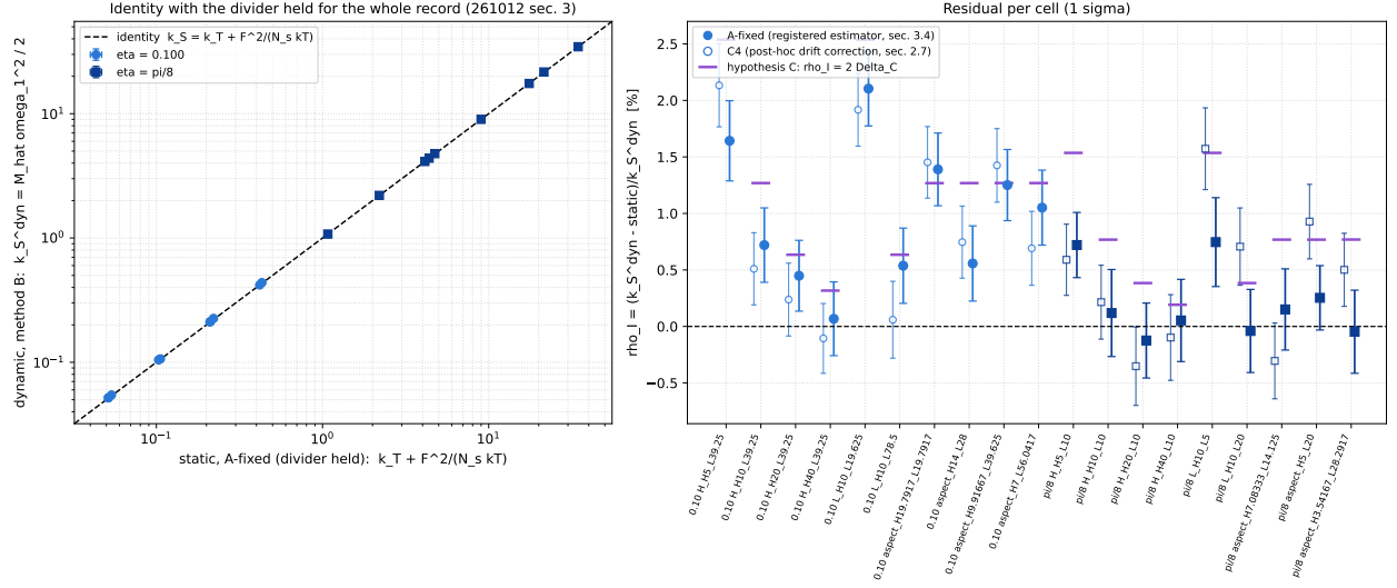
Fig. 10. The static–dynamic identity (7) in 19 boxes. Left: dynamic stiffness (divider mode, heavy masses) against static stiffness (held divider) with the diagonal. Right: the relative residual per cell (filled), the temperature-corrected first measurement (open, see §VII, “The static measurement”), and the residual the anharmonic hypothesis (C) predicts, 2\Delta_C (bars).
