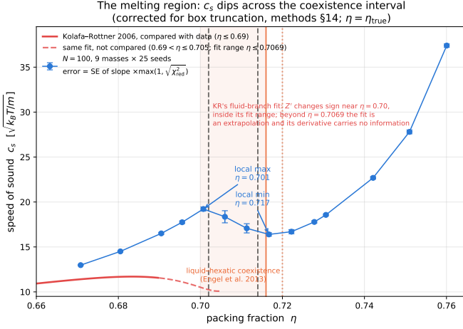
Fig. 12. The melting region. Vertical lines are Engel et al. ’s independently measured landmarks [2]: the Mayer–Wood loop extrema at \eta \approx 0.702 and 0.714 , the end of liquid–hexatic coexistence at 0.716 , and the hexatic–solid crossover at 0.720 . Our c_s turns over inside the same interval. Kolafa–Rottner ( \rho_{\max} = 0.90 fit, fitted to \eta \leq 0.7069 ) is solid where it is compared with data, \eta \leq 0.69 , and dashed from there to \eta = 0.705 , inside its fit range; the fluid-branch fit gives Z' = 48 at \eta = 0.67 , 28 at 0.69 and -9 at 0.700 . Beyond its fit range the fluid-branch fit is an extrapolation and its derivative carries no information. The negative Z' already inside the fit range is also why KR’s own c_s turns over near \eta = 0.683 .
