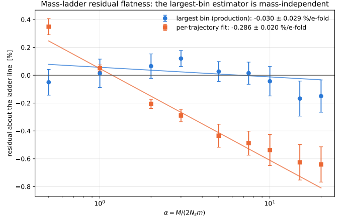
Fig. 5. Mass independence, the ladder’s one assumption, tested. Mean residual about each density’s own ladder line at fixed \alpha = M/2N_s m , averaged over the 24 densities with \eta \leq 0.69 , against \ln \alpha . The largest-bin estimator is flat; the per-trajectory fit drifts by an order of magnitude more per e-fold in \alpha , which is why the largest bin is the production estimator.
