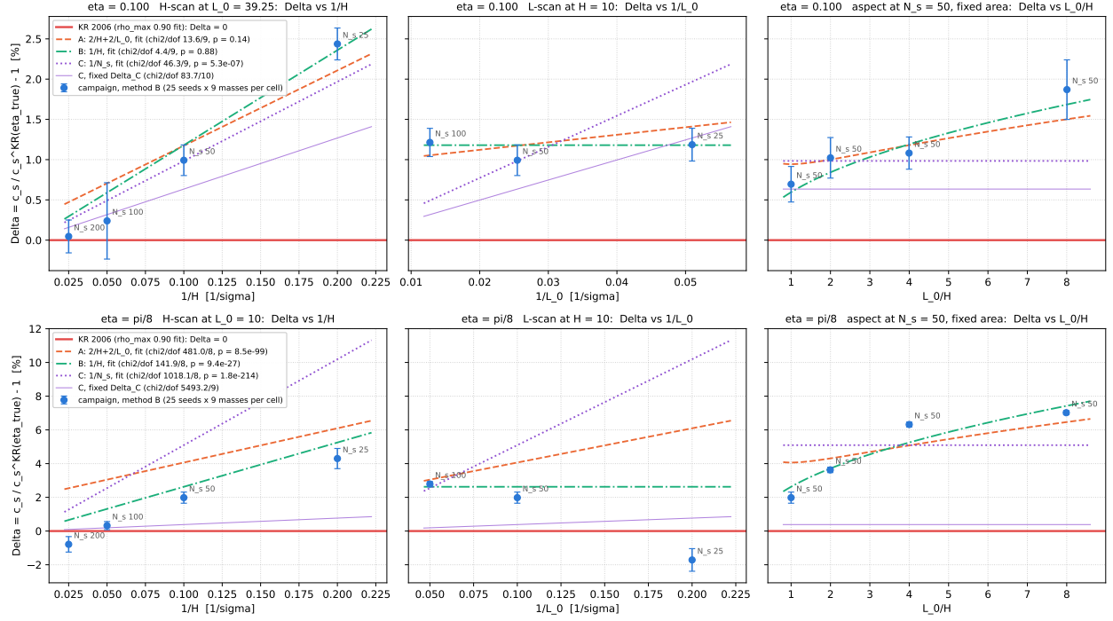
Fig. 9. Confinement shift of the sound speed relative to Kolafa–Rottner (red, \Delta = 0 ). Top \eta = 0.100 , bottom \eta = \pi/8 ; left the height scan against 1/H , middle the length scan against 1/L_0 , right the aspect cells against L_0/H . Lines are the pre-registered forms with their fitted amplitudes. At \eta = 0.100 the data favour the 1/H form ( p = 0.88 ); the pre-registered rule does not exclude 2/H + 2/L_0 ( p = 0.14 ); the 1/N_s form is excluded ( p = 5 \times 10^{-7} ). At \eta = \pi/8 the outcome is not resolved : every form is excluded, and no single-parameter form describes the shape dependence.
