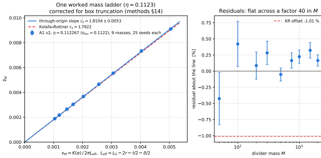
Fig. 4. One worked mass ladder, \eta = 0.1123 , nine divider masses M = 50 –2000, 25 seeds each. Left: \bar{\nu}_M against x_M = K(\alpha)/2\pi L_{\text{eff}} with K the root of \cot K = \alpha K ; the slope through the origin is c_s . Right: residuals about that line, flat across a factor 40 in M . The measured c_s sits 1.0% above Kolafa–Rottner, the finite-size offset discussed in §VI.
