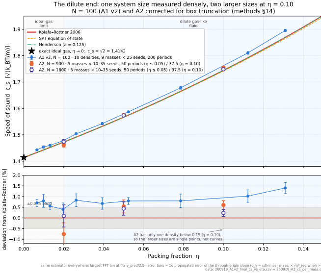
Fig. 7. The dilute end. The N = 100 curve sits 0.4–1.4 % above the equation of state; larger systems agree with it within 2\sigma , except N = 900 at \eta = 0.10 ( 3\sigma ).
