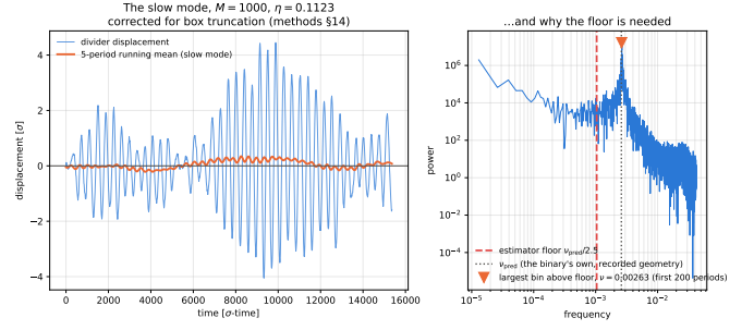
Fig. 2. Why the floor exists. Left: the divider displacement at M = 1000 , \eta = 0.1123 (recorded 0.1122), with its five-period running mean — the slow adiabatic-piston wander, which carries no information about c_s but has more low-frequency power than the resonance. Right: the same record's periodogram. Without a floor the largest bin is the wander, not the mode; the estimator therefore takes the largest bin at f \geq \nu_{\text{pred}}/2.5 .
