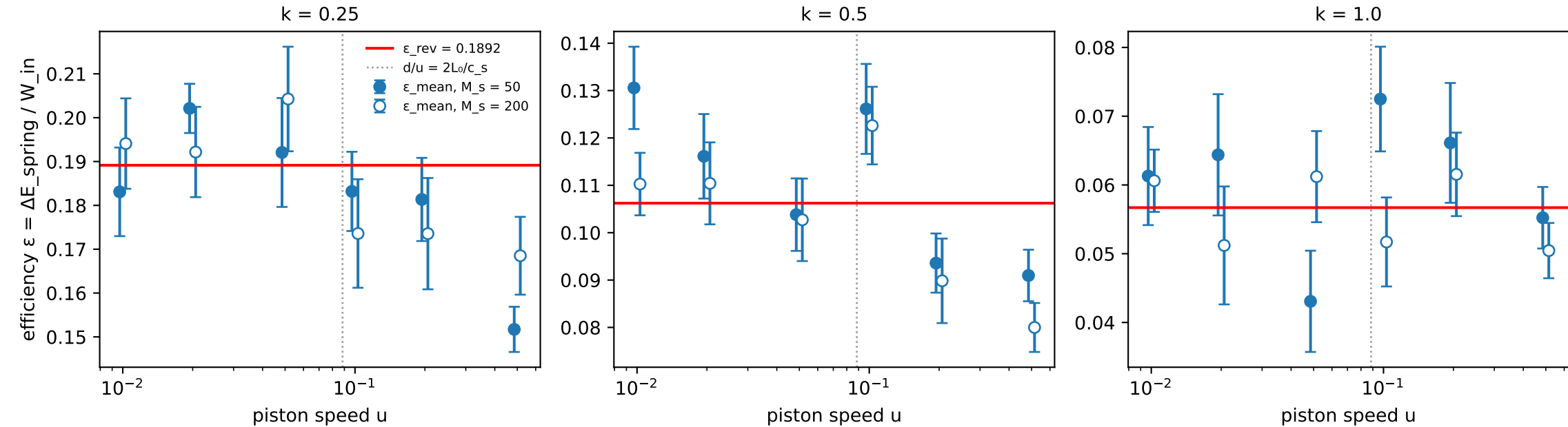
Paper 2 efficiency map, geometry C (shifted \times 0.97/\times 1.03 in u for legibility)
