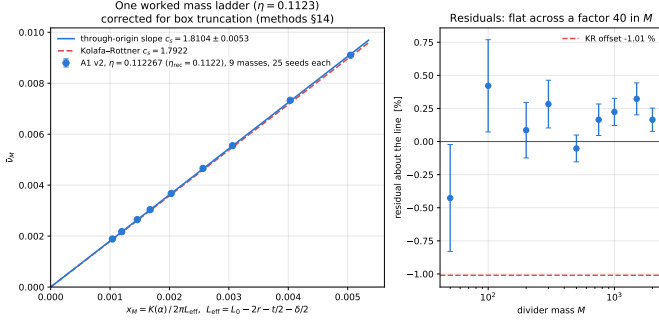
Fig. 4. One worked mass ladder, \eta = 0.1123 , nine divider masses M = 50 –2000, 25 seeds each. Left: \bar{v}_M against x_M = K(\alpha)/2\pi L_{\text{eff}} with K the root of \cot K = \alpha K ; the slope through the origin is c_s . Right: residuals about that line, flat across a factor 40 in M . The measured c_s sits 1.0% above Kolafa–Rottner, the finite-size offset discussed in §VI.
