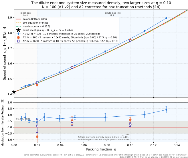
Fig. 7. The dilute end. The N = 100 curve sits 0.4–1.4% above the equation of state; larger systems agree with it within their errors, except N = 900 at \eta = 0.10 ( 3\sigma ).
